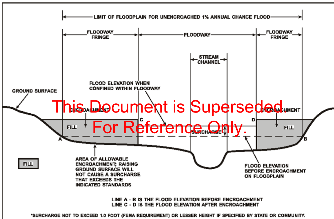
5.2.4 Figure 4, Floodway Schematic
