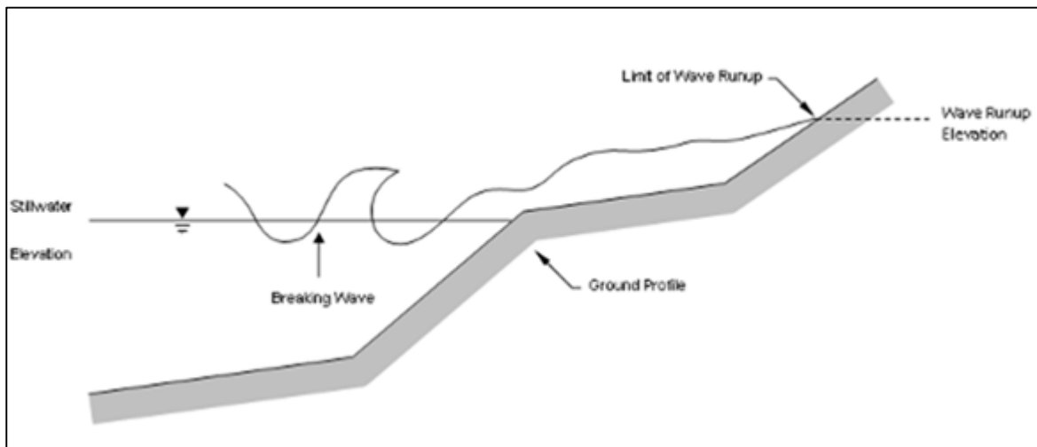
5.2.5 Figure 5, Wave Runup Transect Schematic
