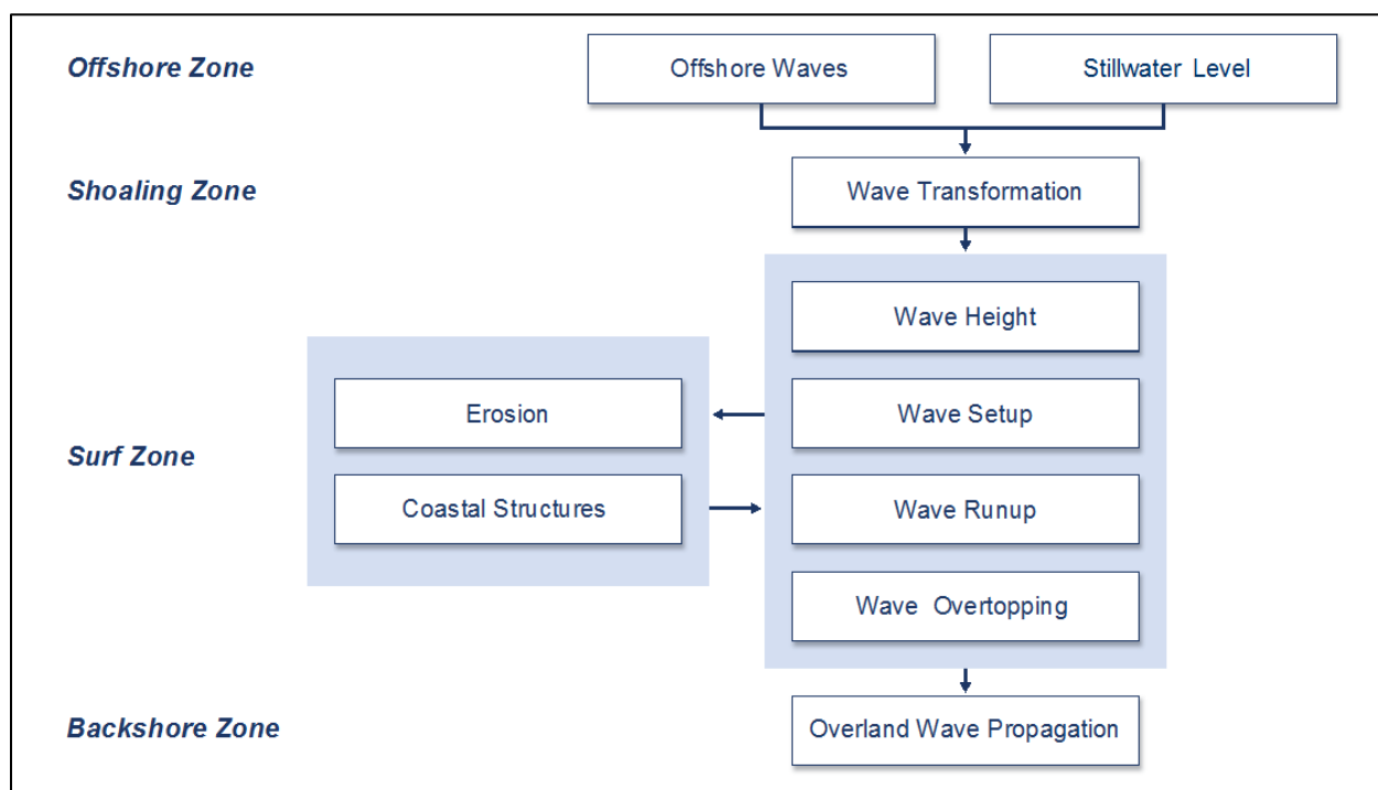
Figure 2: Coastal Processes
