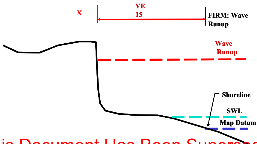
Figure 5-1. Non-erodible High Coastal Bluff with VE Zone Controlled by Wave Runup (No Overtopping)
