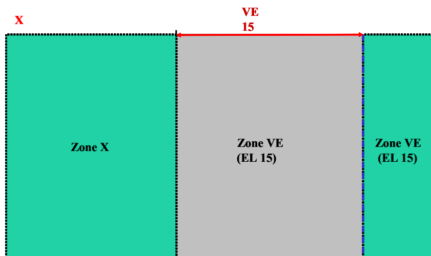
Figure 5-2. Plan View of Flood Hazard Zones and BFEs, Non-erodible High Coastal Bluff with VE Zone Controlled by Wave Runup (No Overtopping)
