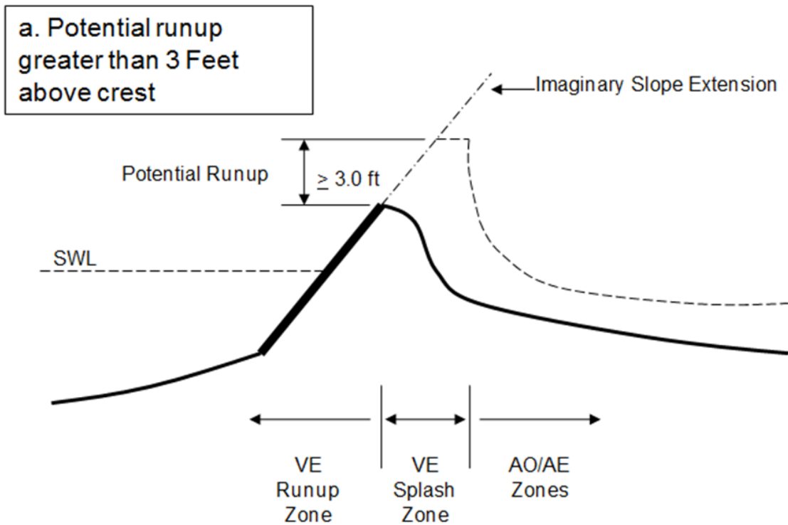
Figure 2-2. Simplified Mapping Procedure for Overtopped Barrier
