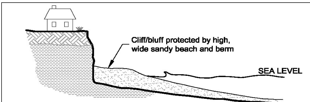
Figure 6: Example of Sandy Beach Backed by Bluff
