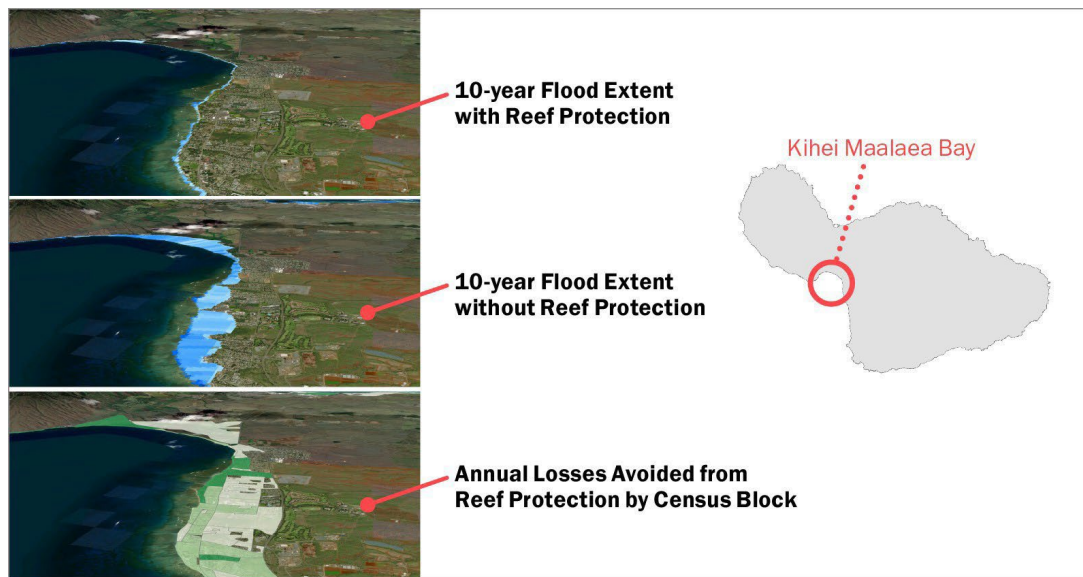
Figure 5-19. Risk Reduction Benefits of Coral Reefs on Maui – Kihei (Changes in flood extent and annual flood losses avoided due to coral reef protection at Kihei Maalaea Bay Identified as optimal for reef mitigation investment by a hot spot analysis)
