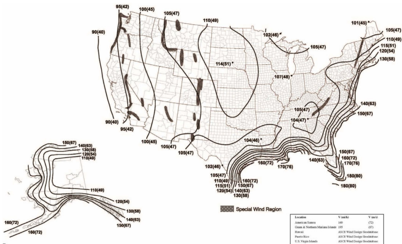
Figure 0.0.5. ASCE 7-22 Hurricane-Prone Region.
