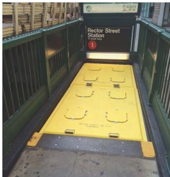
Figure 5.2.6. Deployable covers for subway access stairways can help prevent flooding of underground stations. (Source: Metropolitan Transportation Authority, 2021)
