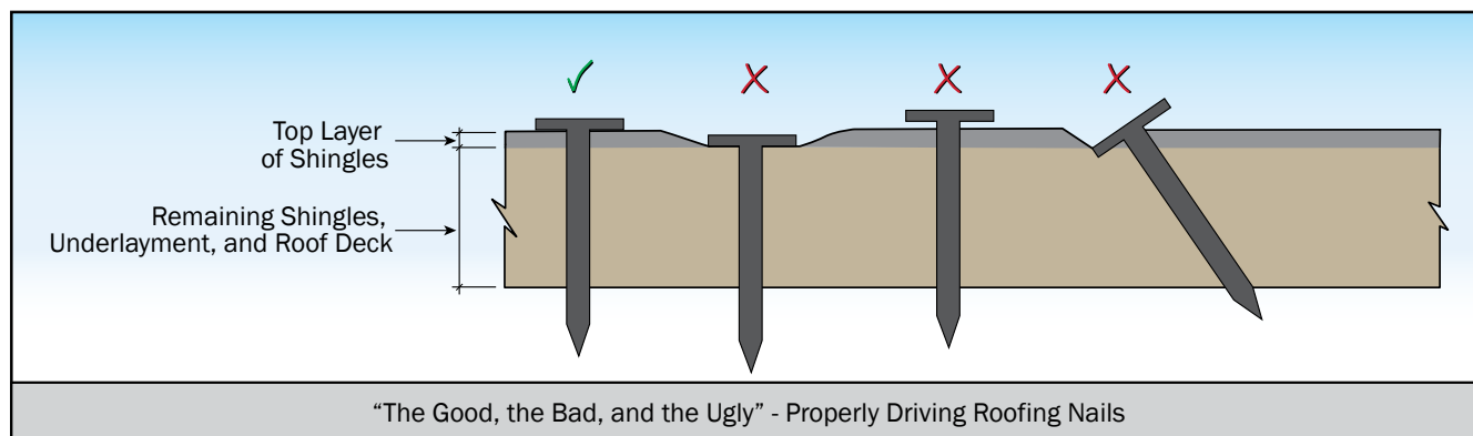
Figure 3.3.1.8. The Dos and Don'ts of driving roof nails through asphalt shingles.
