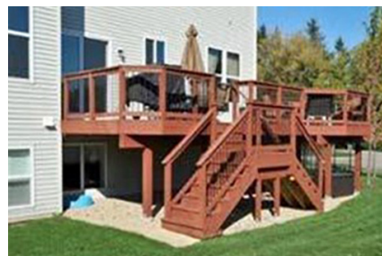
▲ A deck with two sets of stairs; only one is covered for egress.
