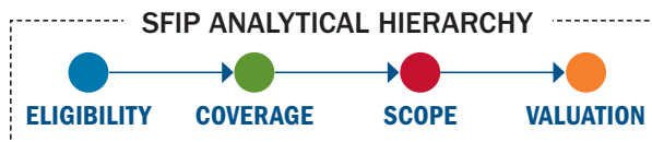
FIGURE 3: SFIP HIERARCHY
