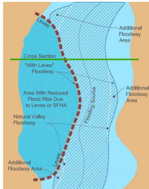
Figure 28: Final Regulatory Floodway
