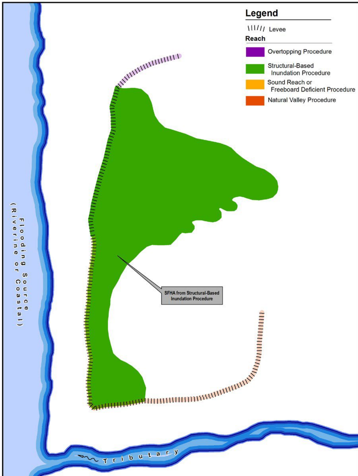
Figure 20: SFHA Delineation Using Structural-Based Inundation Procedure
