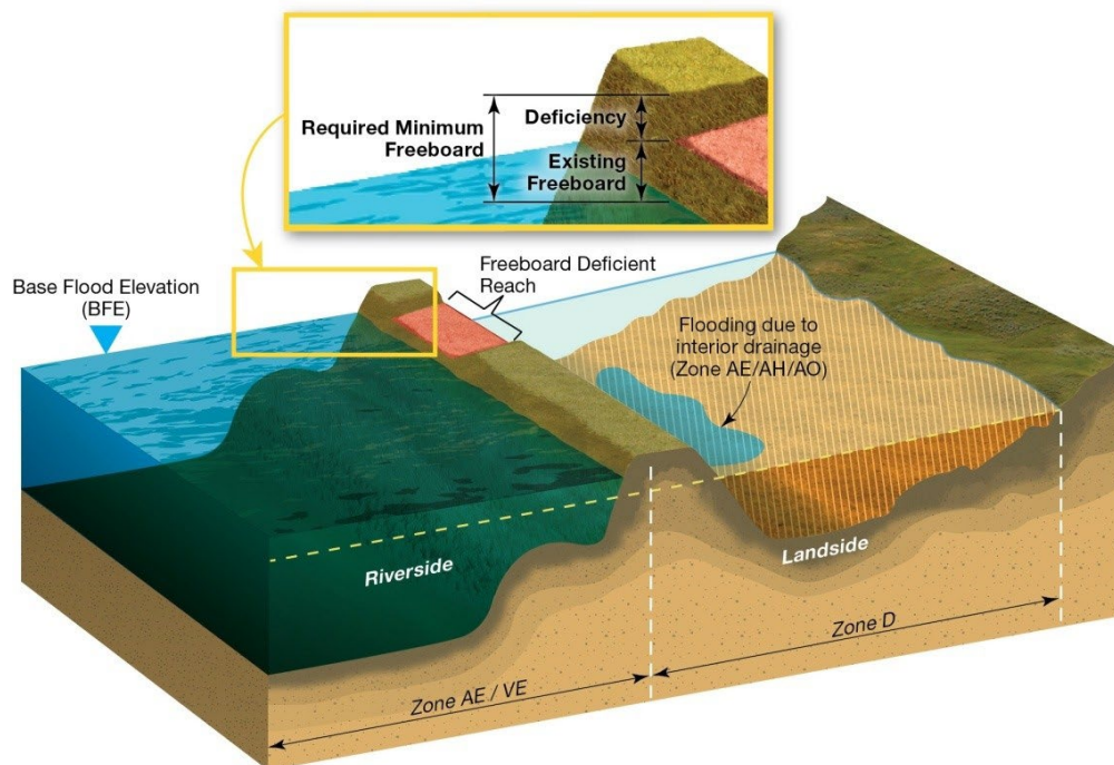
Figure 23: Freeboard Deficient Cross-Section View
