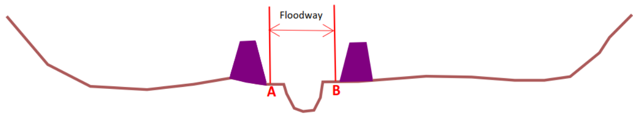
Figure 29: Both Encroachments (A and B) on Riverside of Levees
