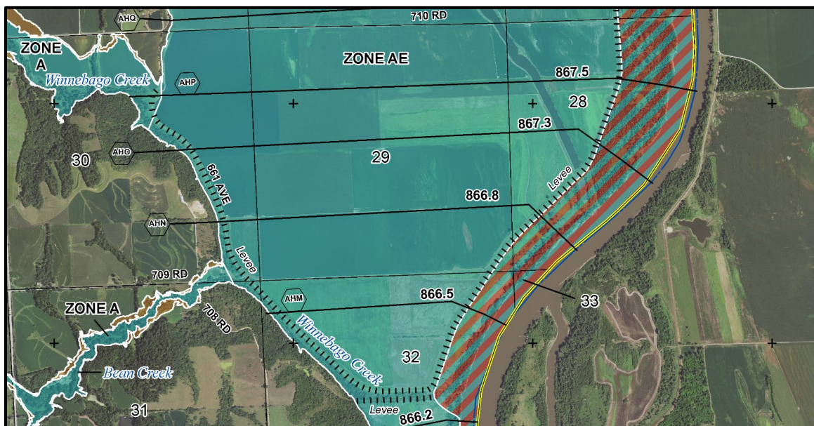
Figure 41: Flood Hazard Mapping for Non-Accredited Levee System
