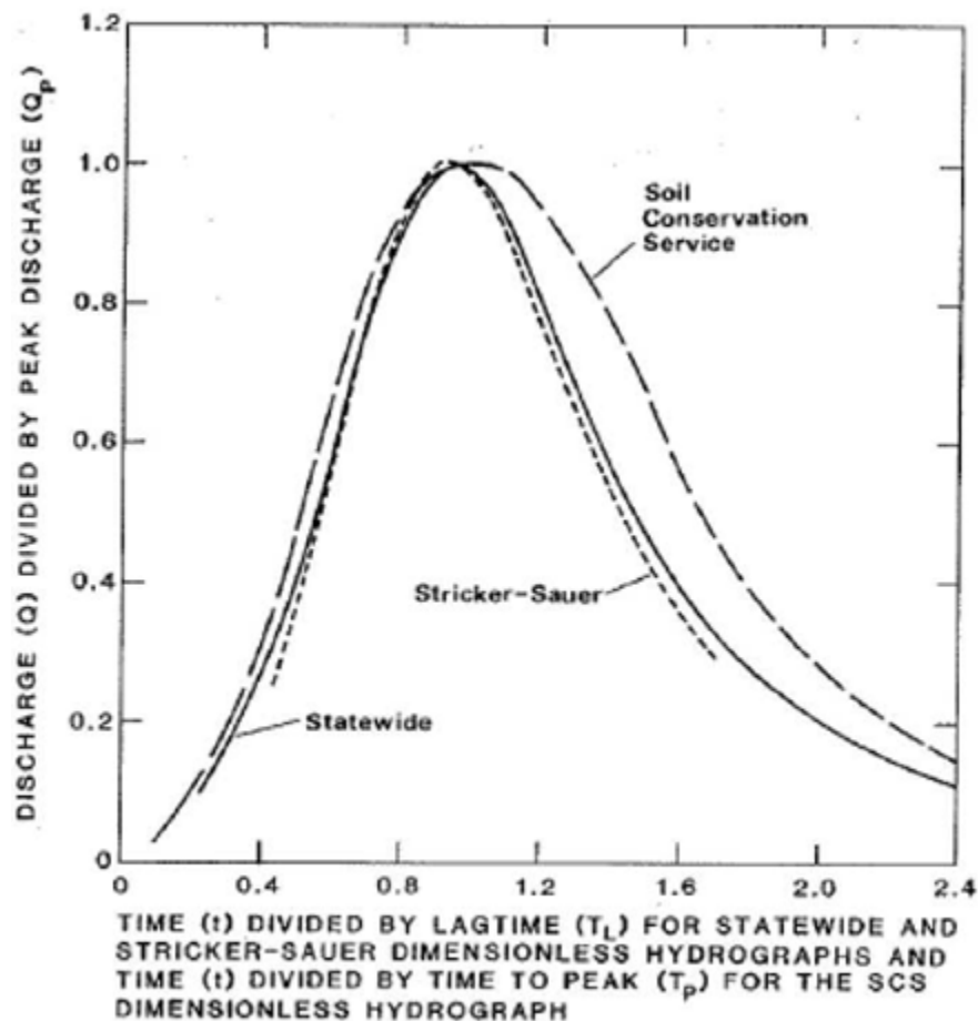
Figure 25: Sample Dimensionless Unit Hydrograph
