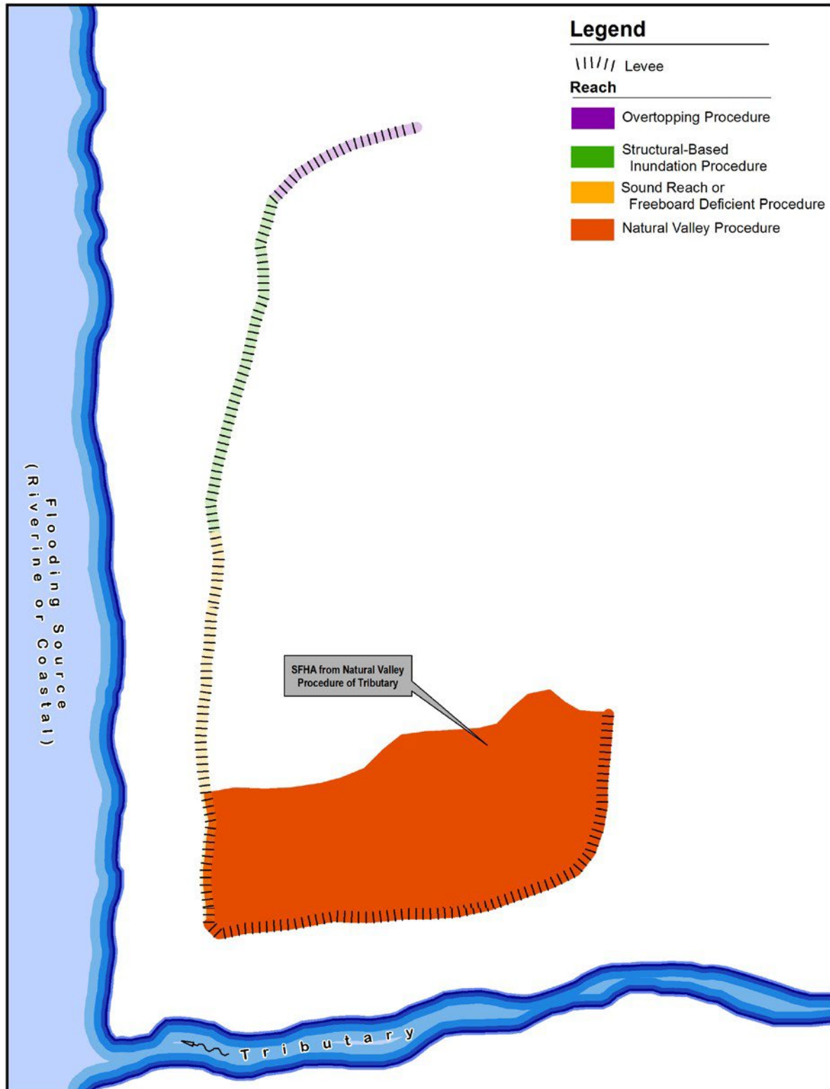
Figure 18: SFHA Delineation Using Natural Valley Procedure
