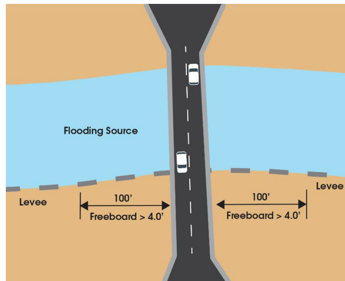
Figure 4: Freeboard Near Structures
