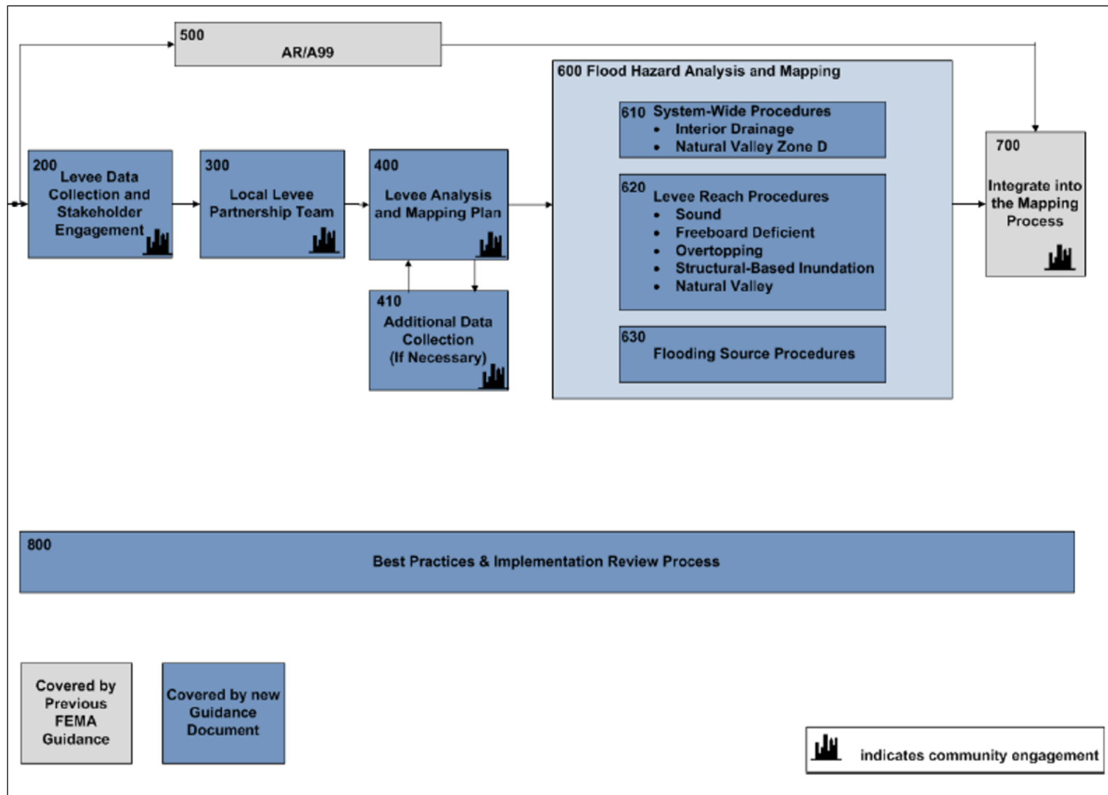
Figure 13: FEMA Levee Analysis and Mapping Procedure
