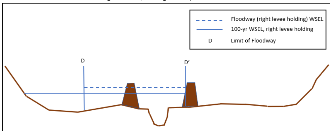
Figure 36: Right Levee Holding to Find Encroachment Station D
