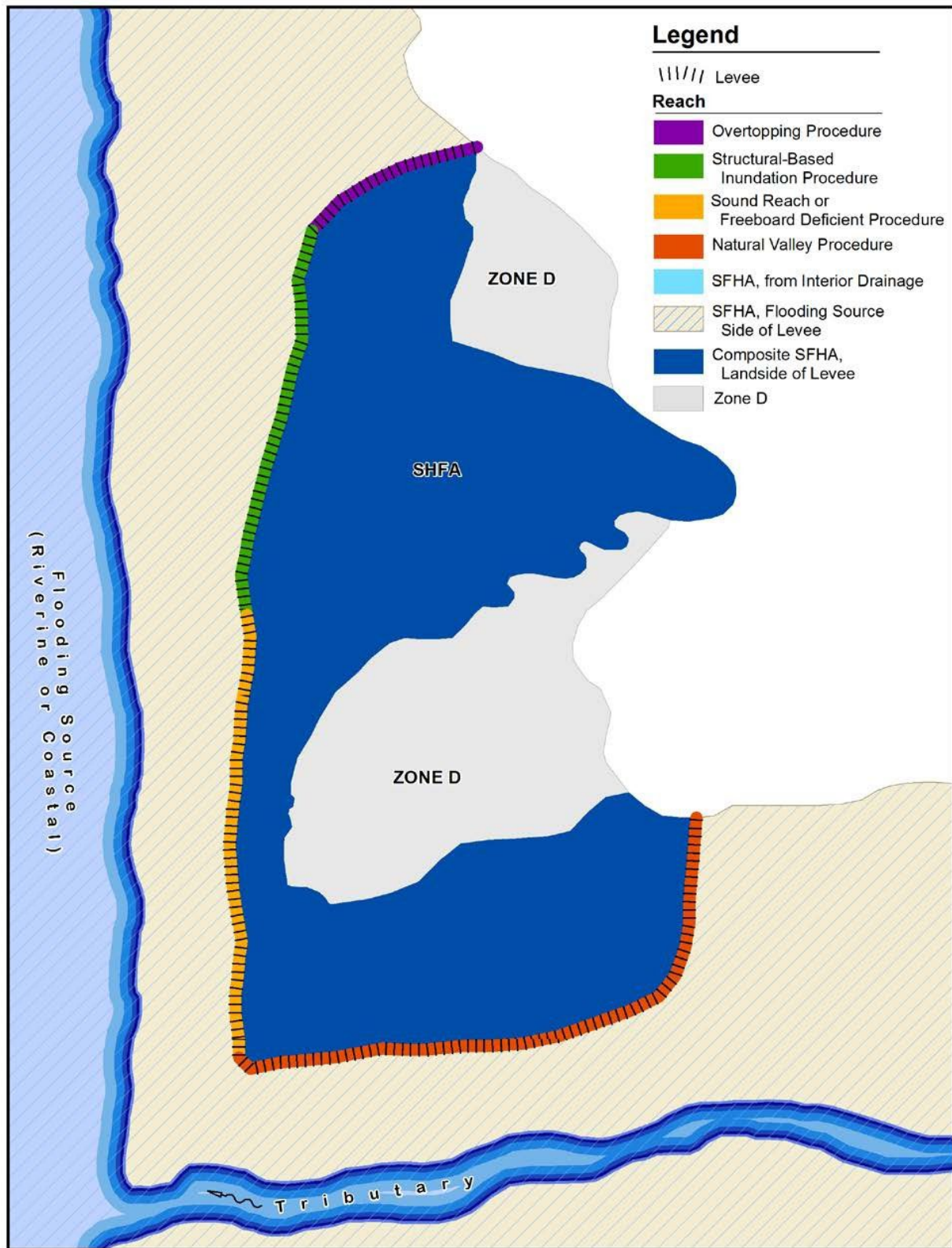
Figure 40: Composite Mapping of Flood Hazards for the Levee System
