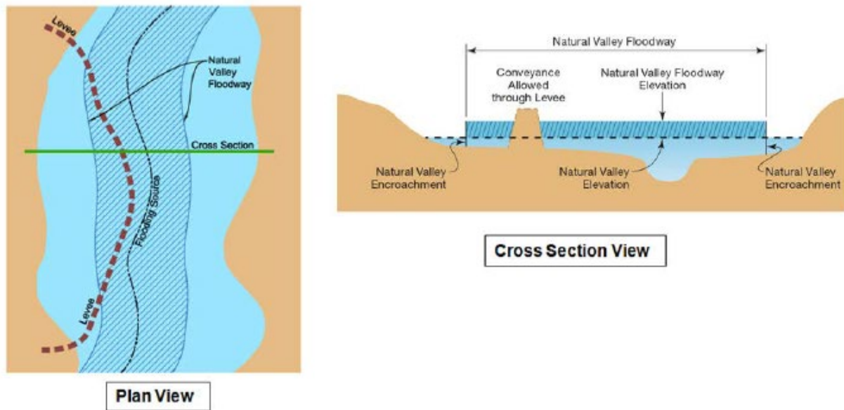
Figure 26: Floodway Analysis Process Initial Analysis
