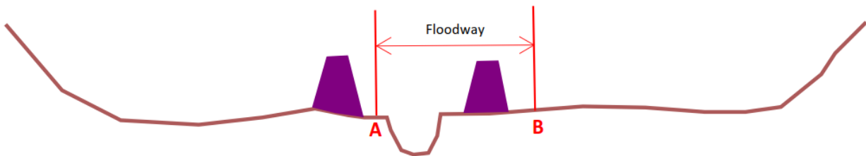
Figure 30: One Encroachment on Riverside of Levee (A) and the Other on Landside of Levee (B)
