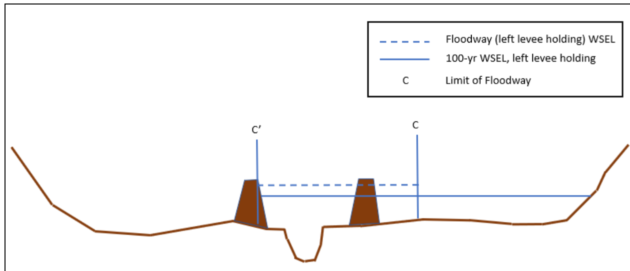
Figure 35: Using Left Levee Holding to Find Encroachment Station C
