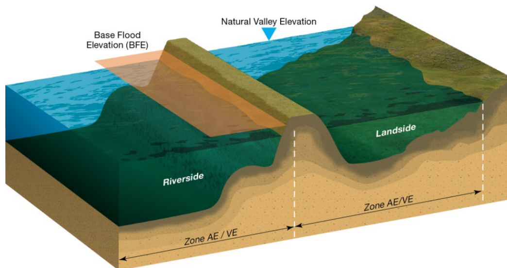
Figure 17: Natural Valley Cross-Section View
