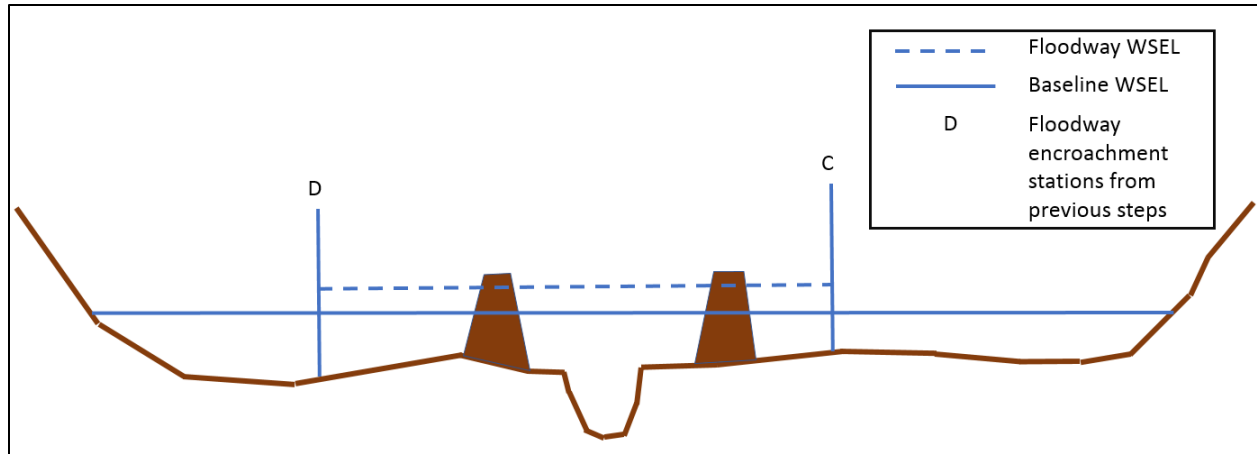
Figure 37: Both levees Are Non-accredited
