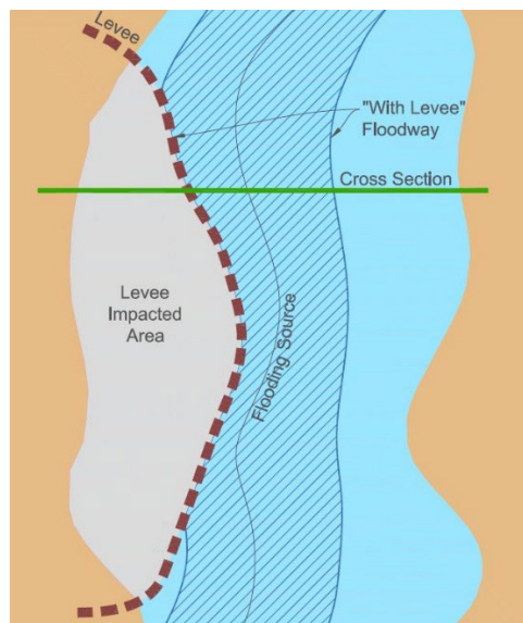
Figure 27: Floodway Analysis Process Initial Analysis
