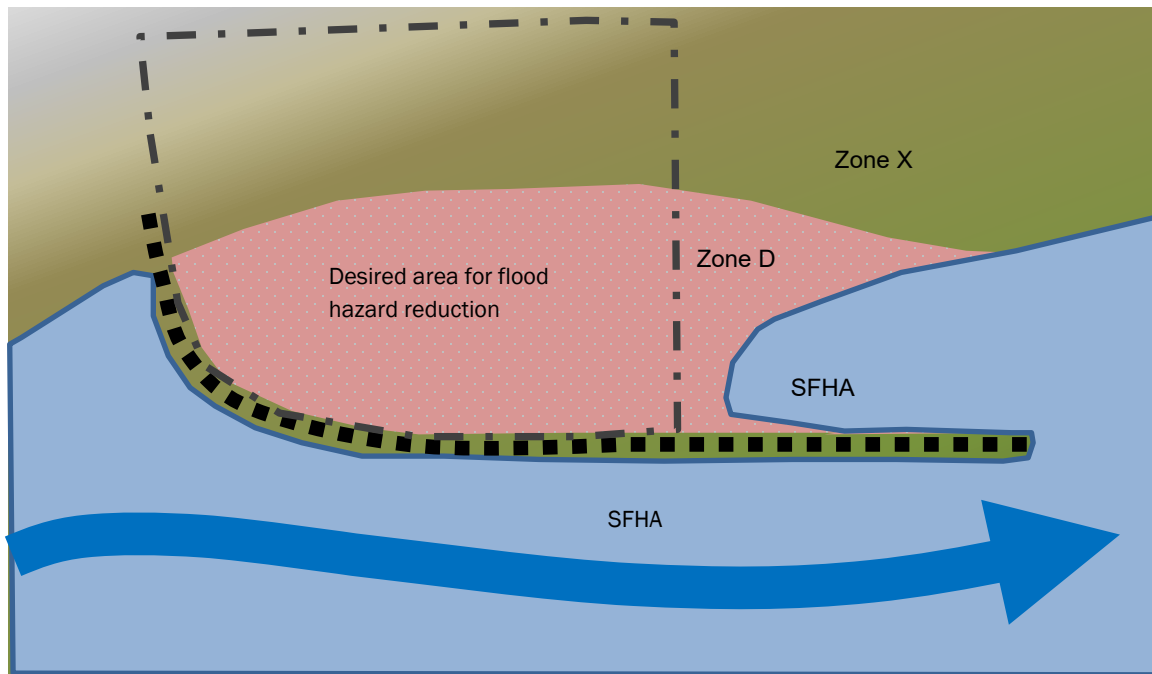
Figure 8: Non-Accredited Levee System
