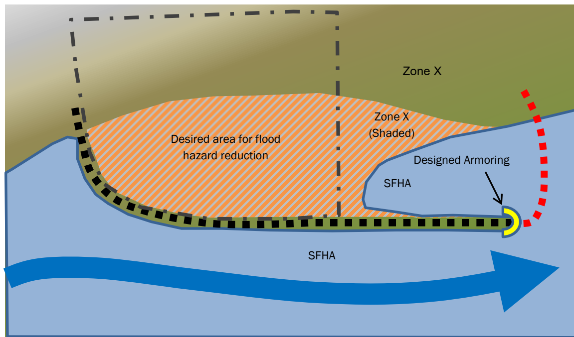
Figure 7: Levee System Tying into Non-Levee Reach
