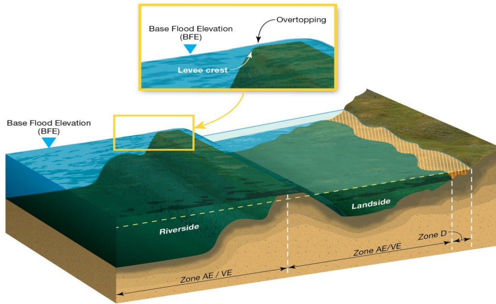
Figure 21: Overtopping Cross-Section View
