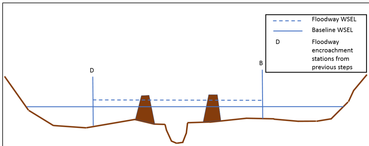
Figure 38: Left Levee Is Non-accredited, Right Levee Is Accredited
