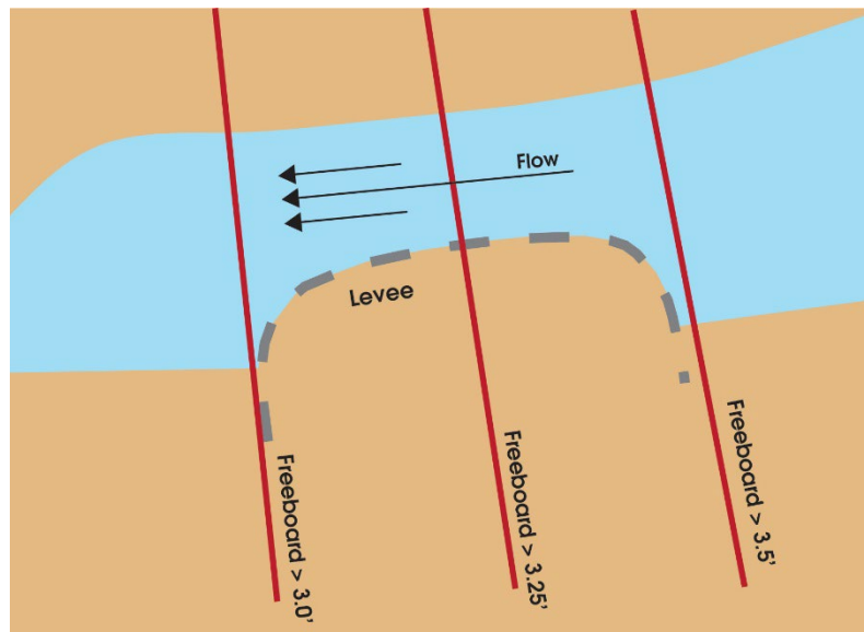
Figure 3: Freeboard Determination
