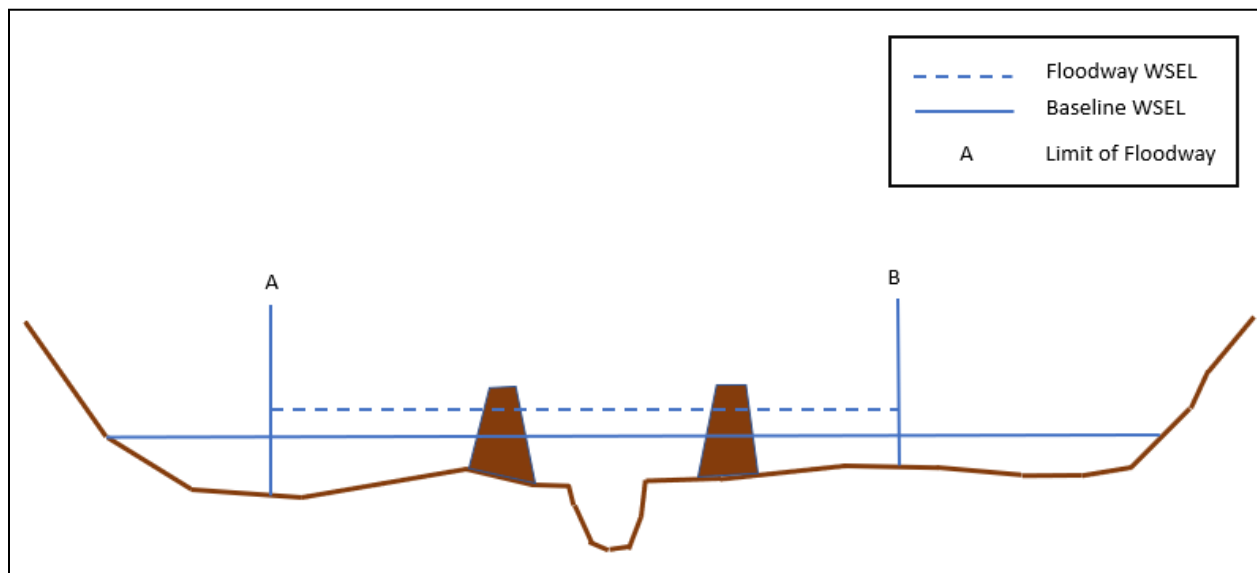
Figure 34: Use of Natural Valley Procedure to Determine Initial Encroachment Stations A and B
