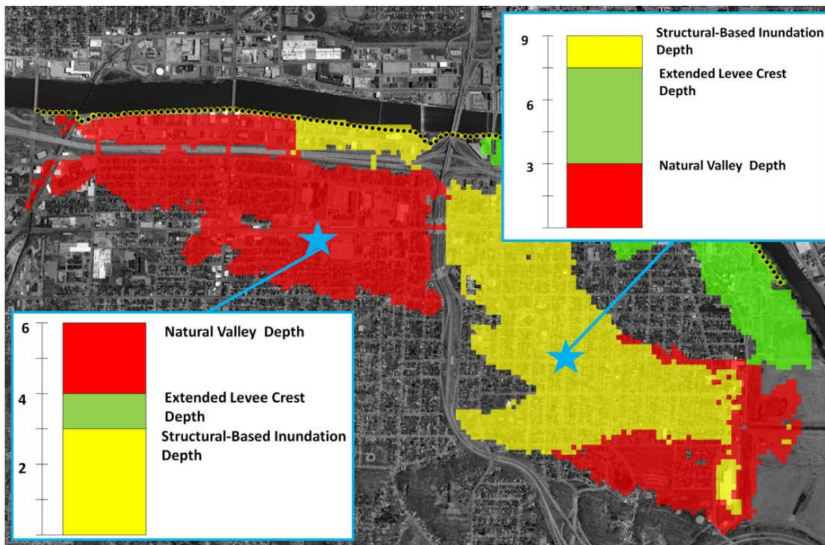
Figure 15: Sample of Potential Inundation Extents
