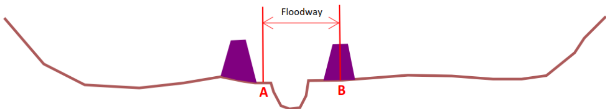
Figure 31: The Landside Encroachment (B) Moved to the Levee
