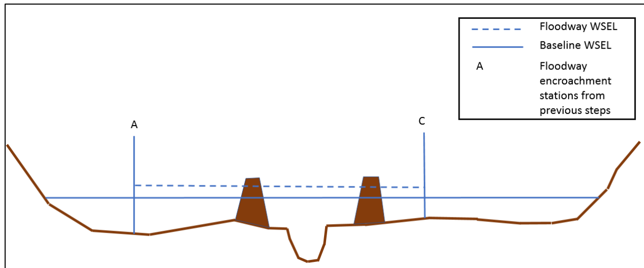
Figure 39: Right Levee Is Non-accredited, Left levee Is Accredited
