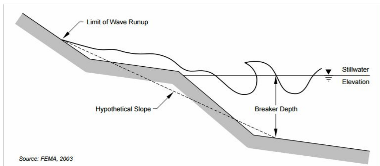
Figure 5: Wave Runup
