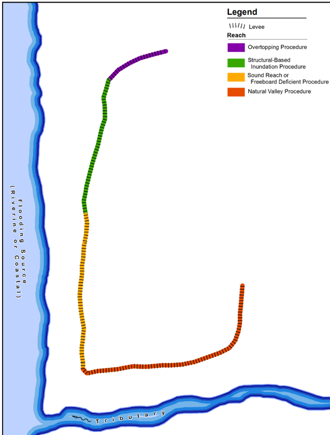
Figure 16: Example Segmentation of a Levee System
