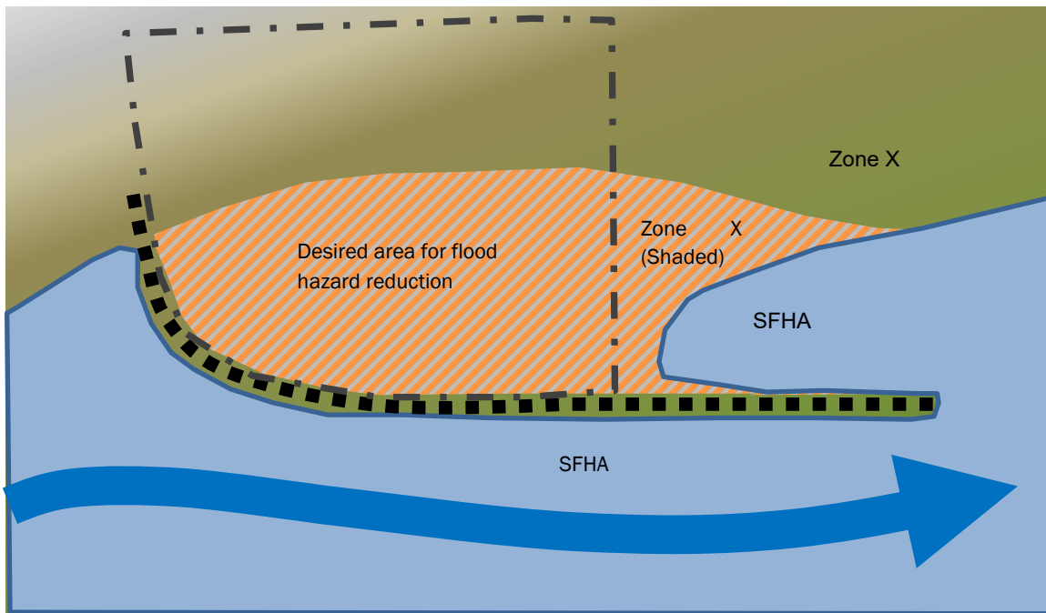
Figure 6: Levee System Designed to End in the Absence of High Ground
