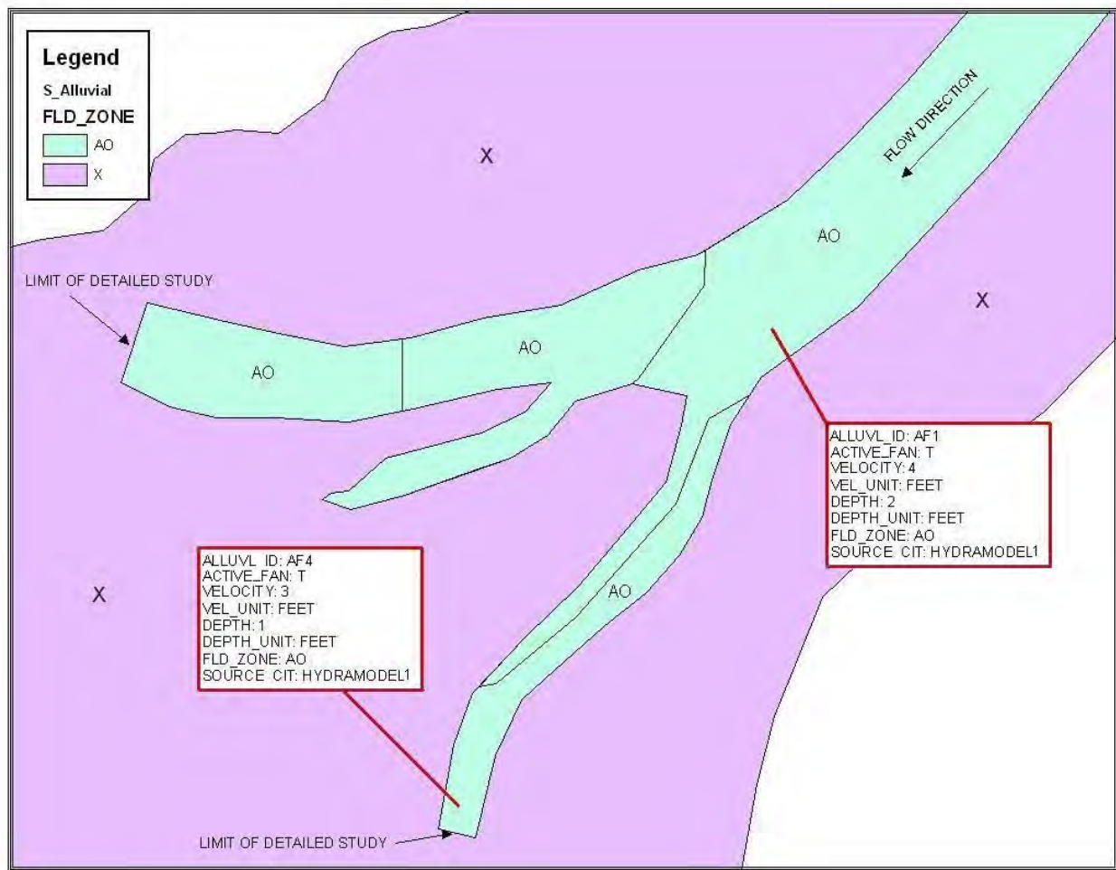
Figure 2: S_Alluvial_Fan
