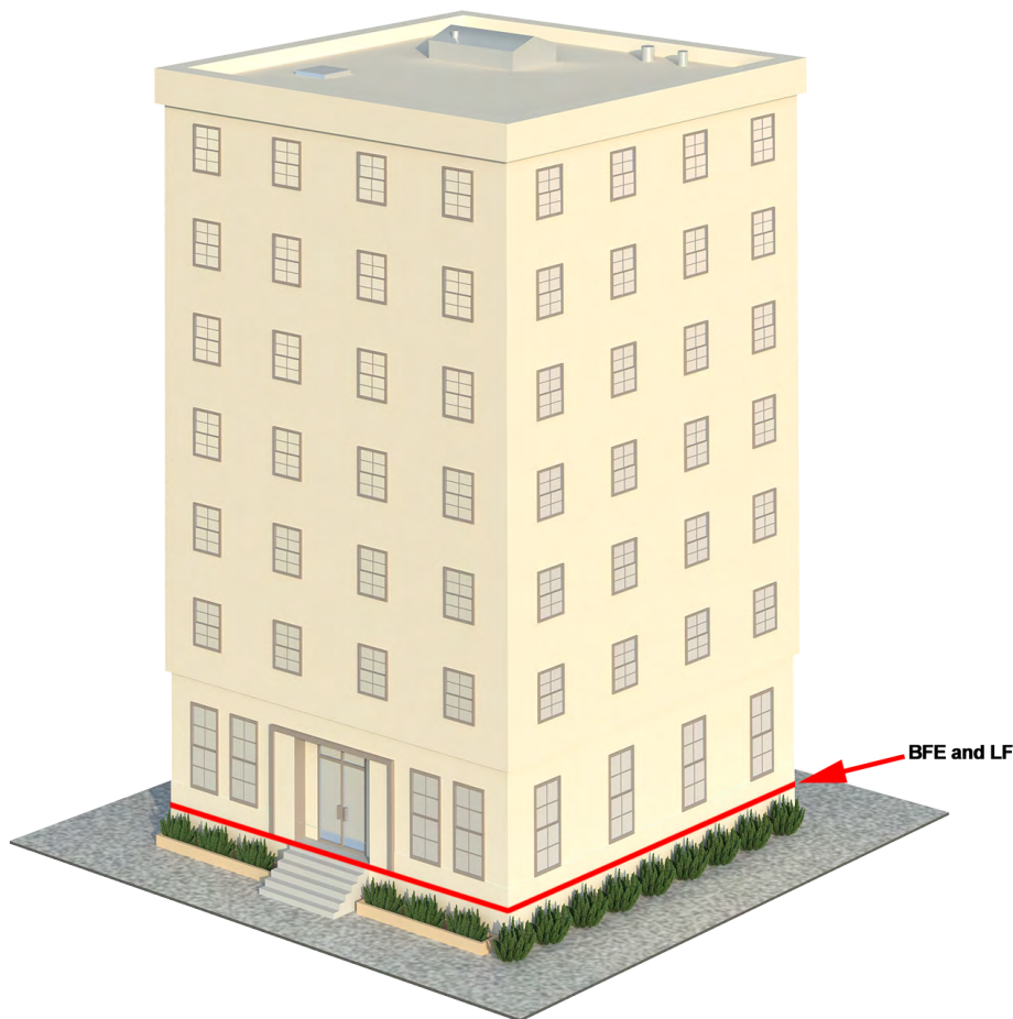
Figure 2-2. Example of a multi-family building constructed to a compliant elevation
