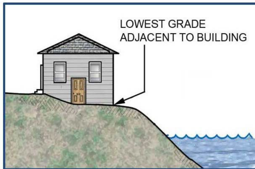
Figure 2: LAG - Lowest Ground Touching a Structure
