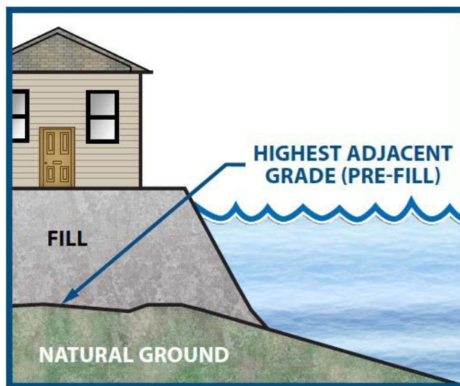
Figure 19: HAG for a Structure
