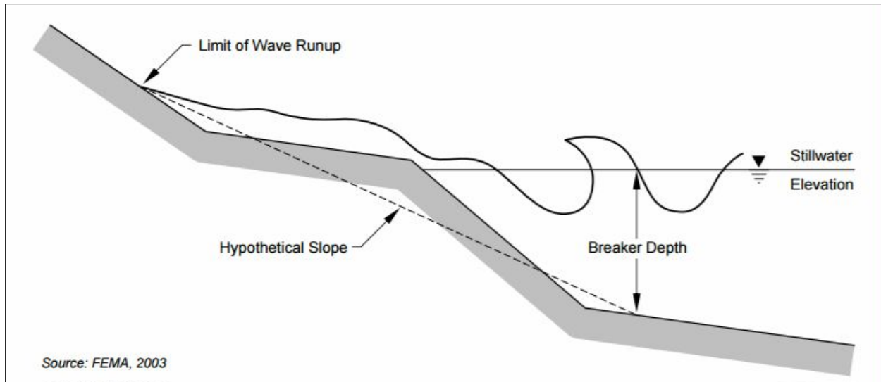
Figure 4: Wave Runup
