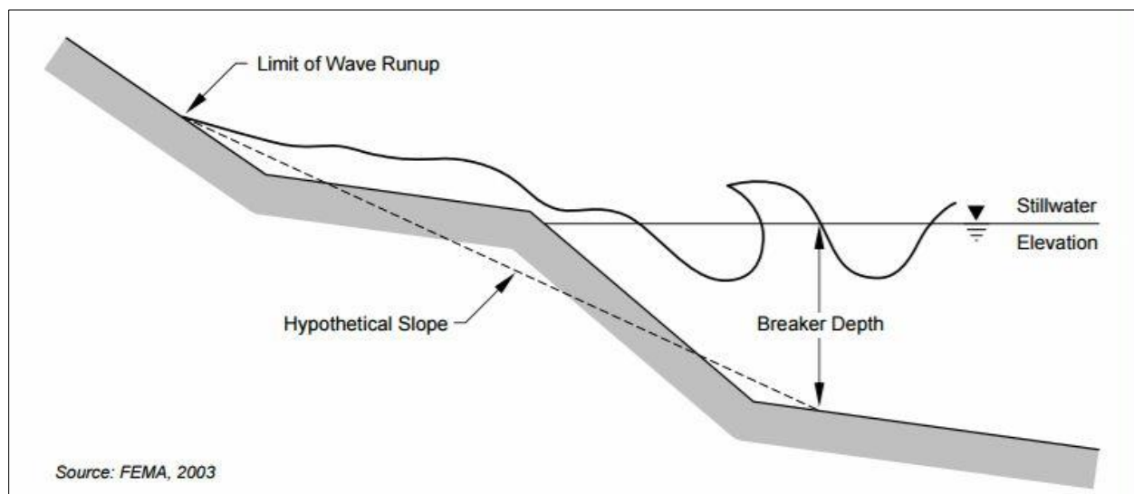
Figure 4: Wave Runup
