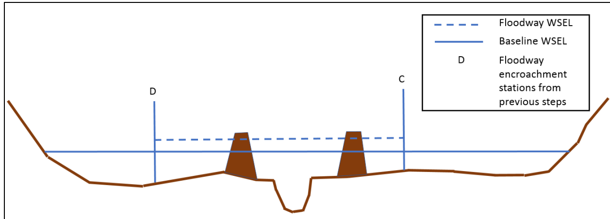
Figure 36: Both levees Are Non-accredited
