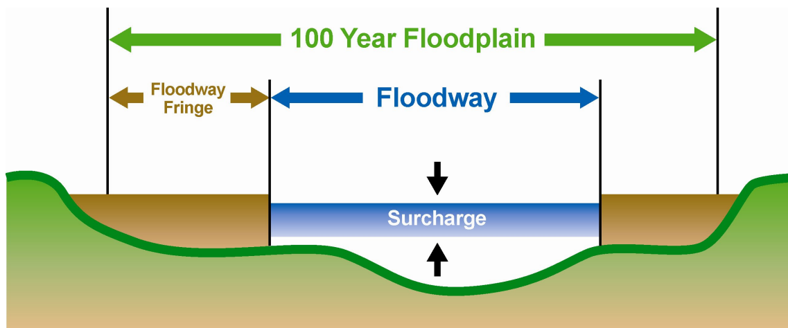
Figure 2. Cross section of a floodplain showing the floodway, floodway fringe, and surcharge
