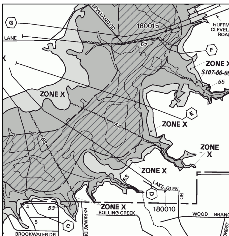
Figure 1. An example of a Flood Insurance Rate Map showing the floodway, cross section locations, and base flood elevations
