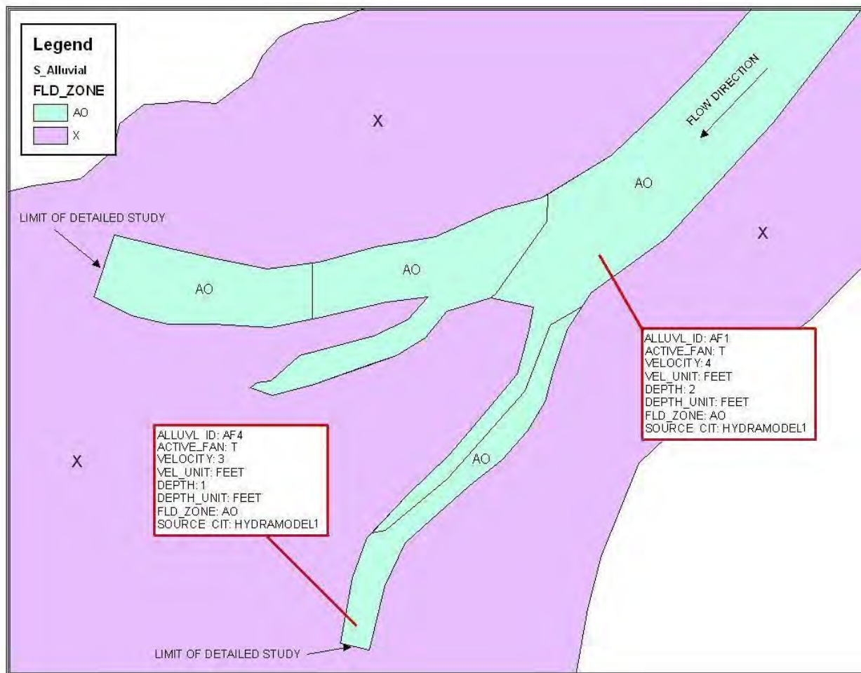
Figure 2: S_Alluvial_Fan
