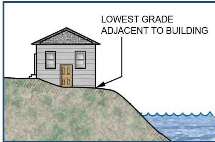
Figure 1: LAG - Lowest Ground Touching a Structure This document has been superseded. For reference only
