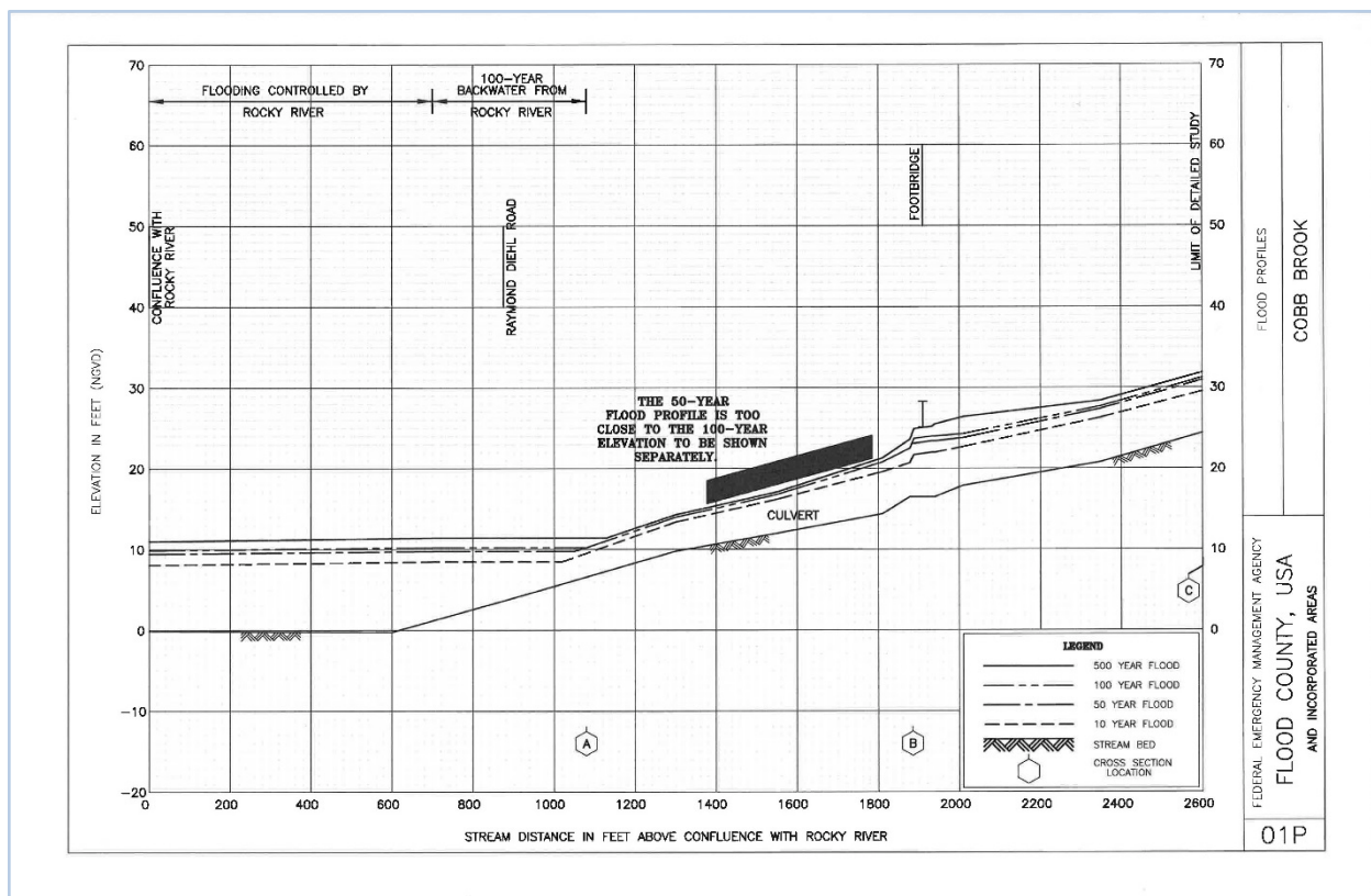
This document has been superseded. For reference only Figure 7. Example of Stream Profile from FIS Report
