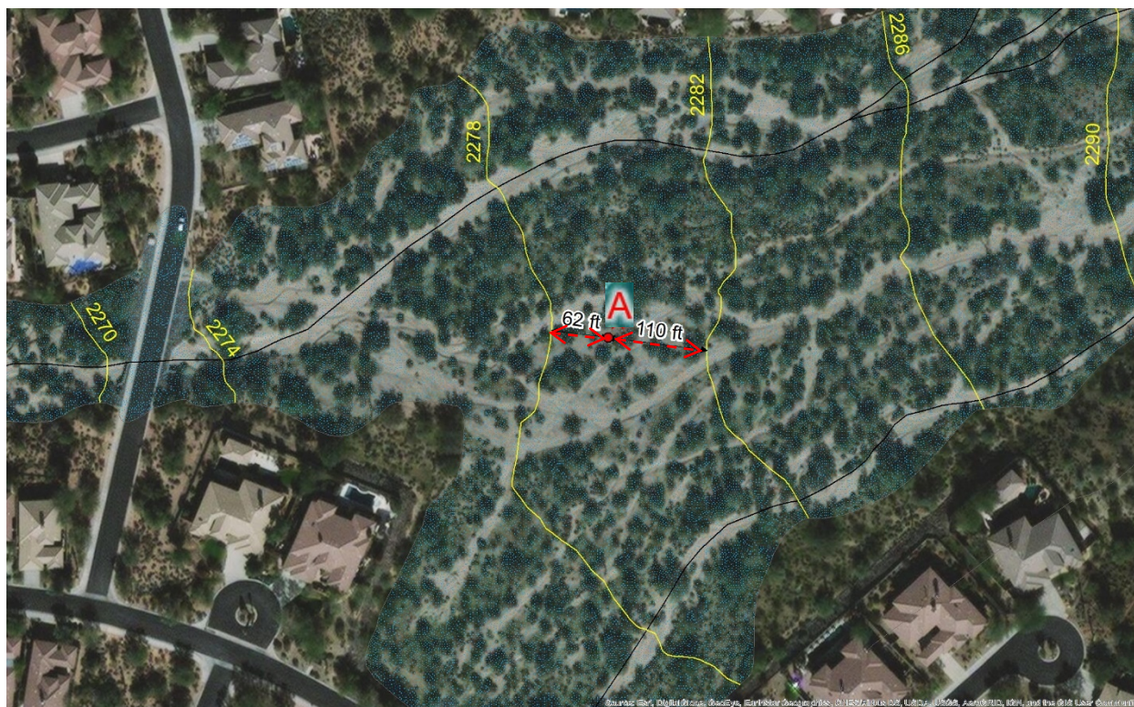
Figure 10: Measuring a Subject between BFEs in overbank areas when the floodplain is derived from 2-D models.
