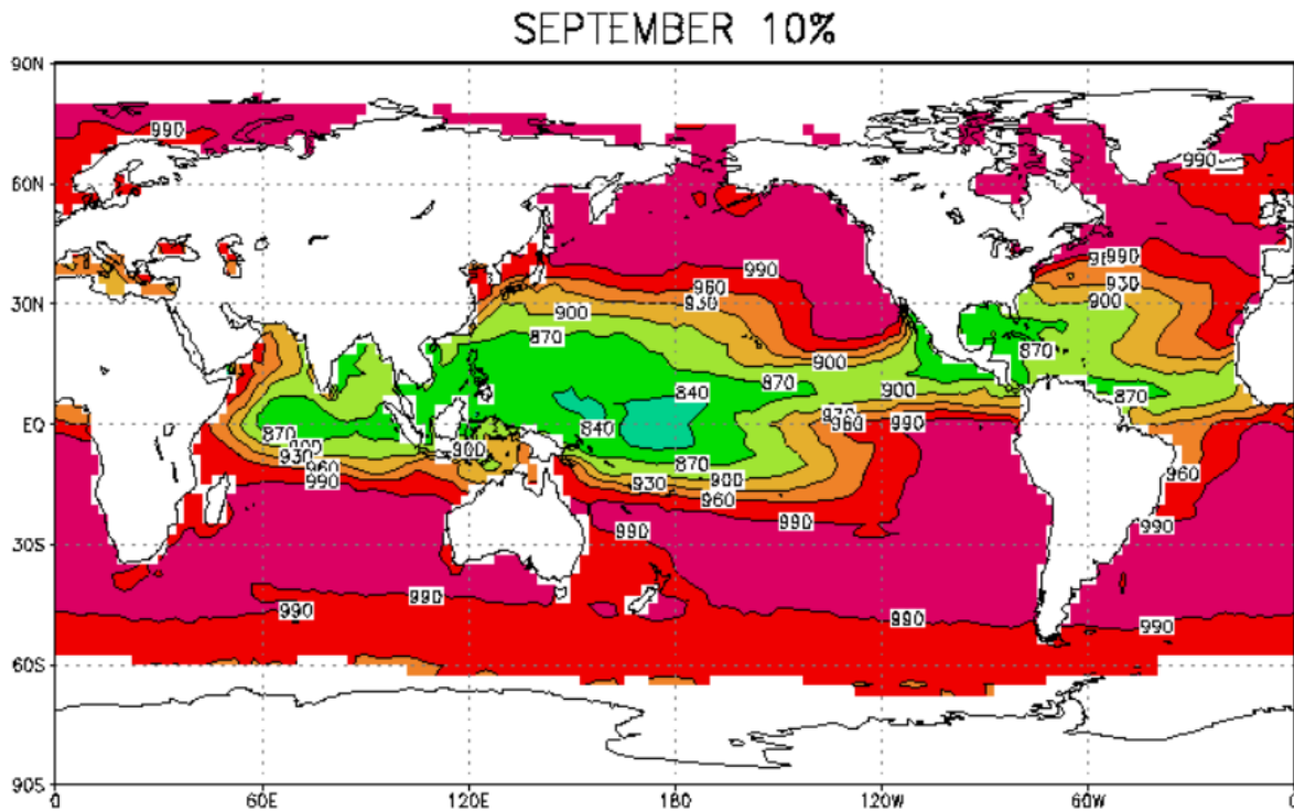
Figure 10-15 10% Exceedance probability maximum potential intensity at a point based on central pressure (hPa) within 621 miles (1000 km) of the point in question for September.
