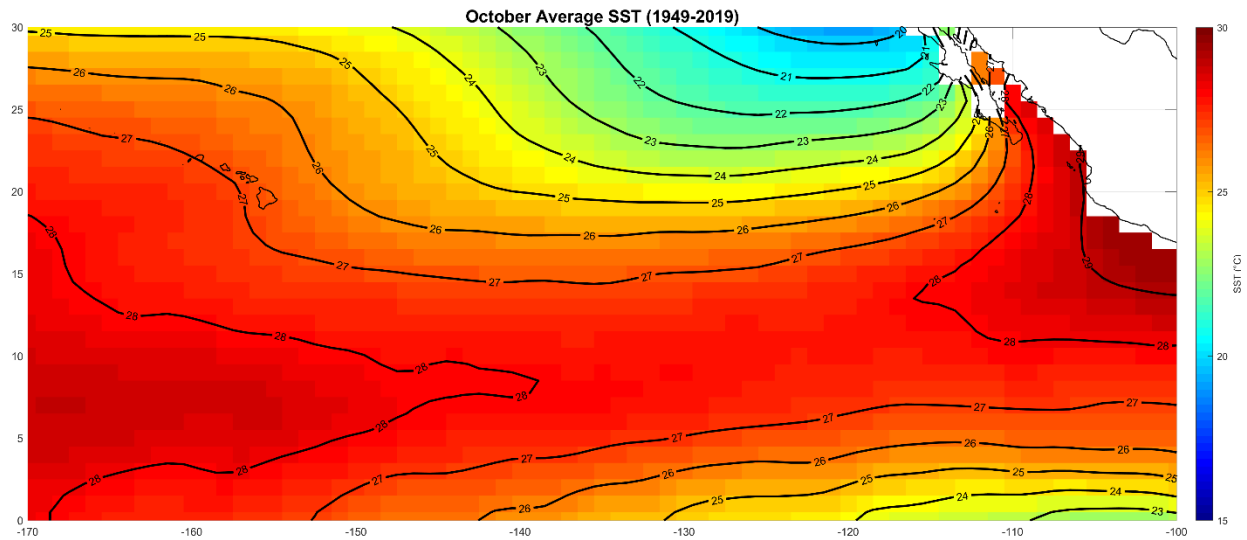
Figure 10-9 Mean October sea-surface temperature (°C)
