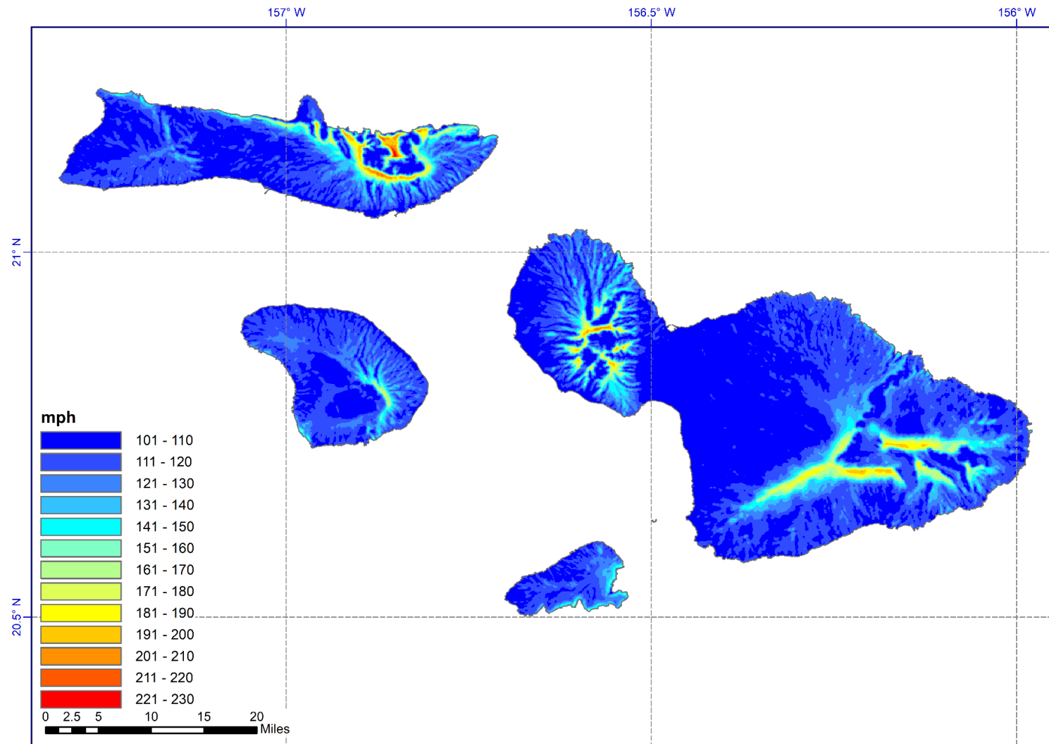
Figure 10-43 Peak gust wind speed map for a return period of 700-years for the islands of Maui, Molokai, Lanai, and Kaho'olawe. Modeled gust wind speeds include the effects of topography.
