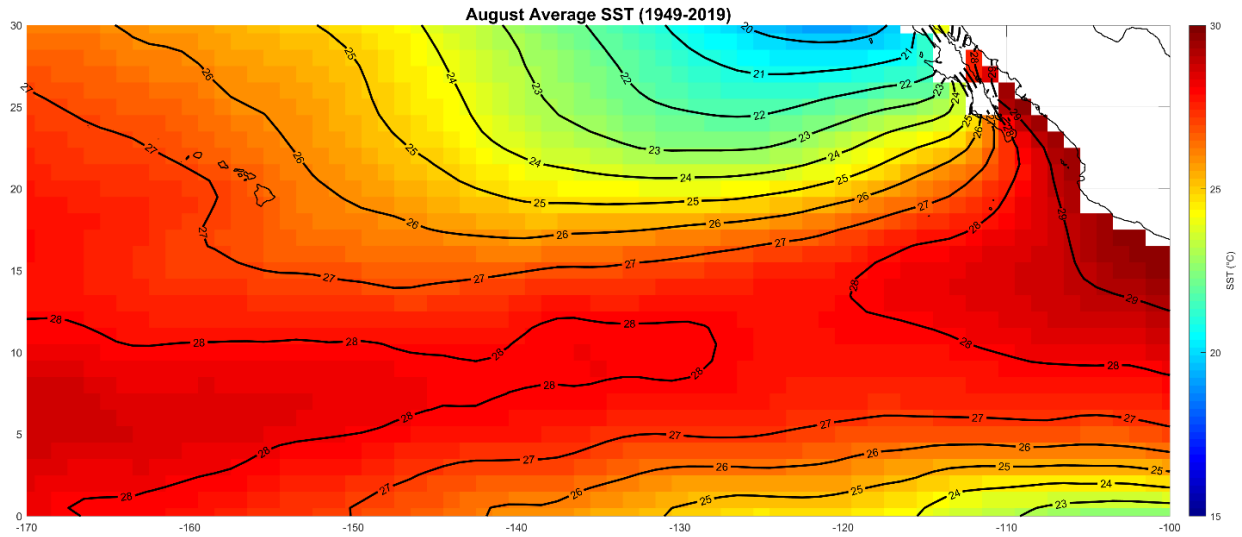
Figure 10-7 Mean August sea-surface temperature (°C)
