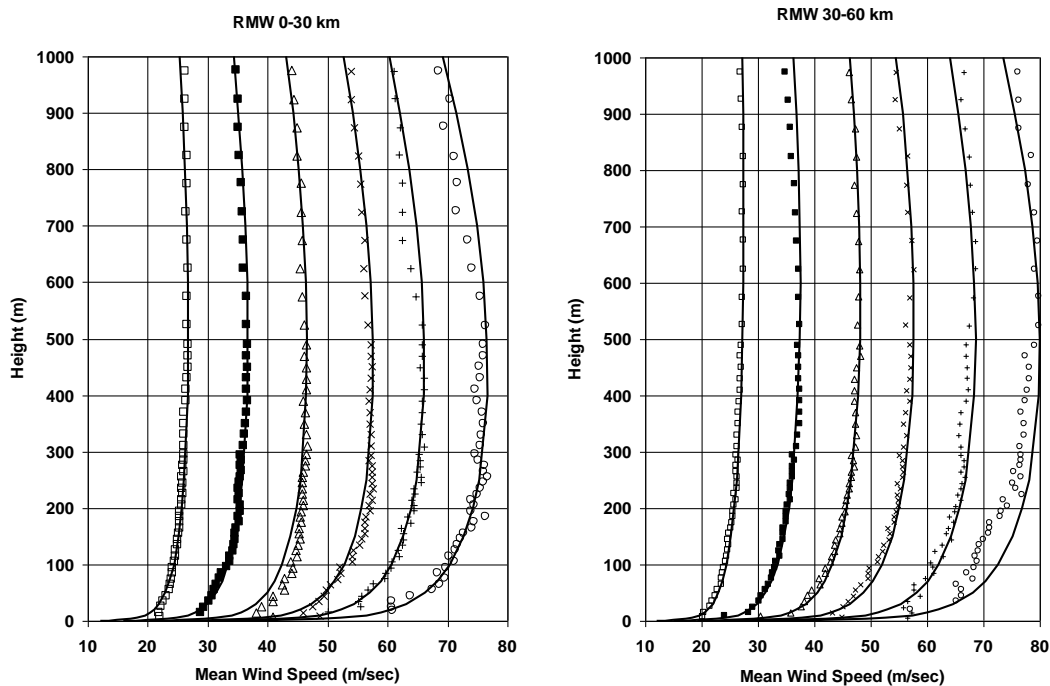
Figure 10-36 Modeled and observed hurricane mean vertical profiles of horizontal wind speed over the open ocean for a range of wind speeds.
