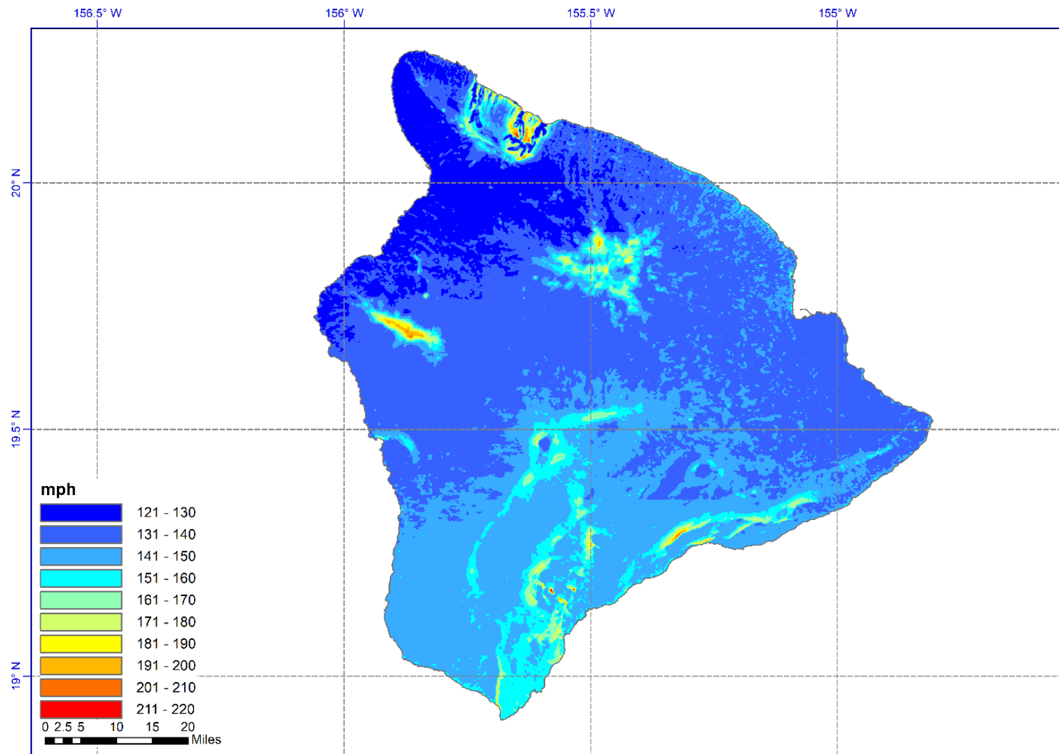
Figure 10-46 Peak gust wind speed map for a return period of 3,000-years for the island of Hawaii. Modeled gust wind speeds include the effects of topography.
