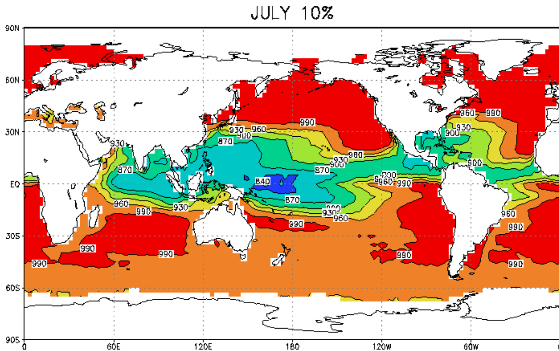
Figure 10-11 10% Exceedance probability maximum potential intensity at a point based on central pressure (hPa) within 621 miles (1000 km) of the point in question for July.
