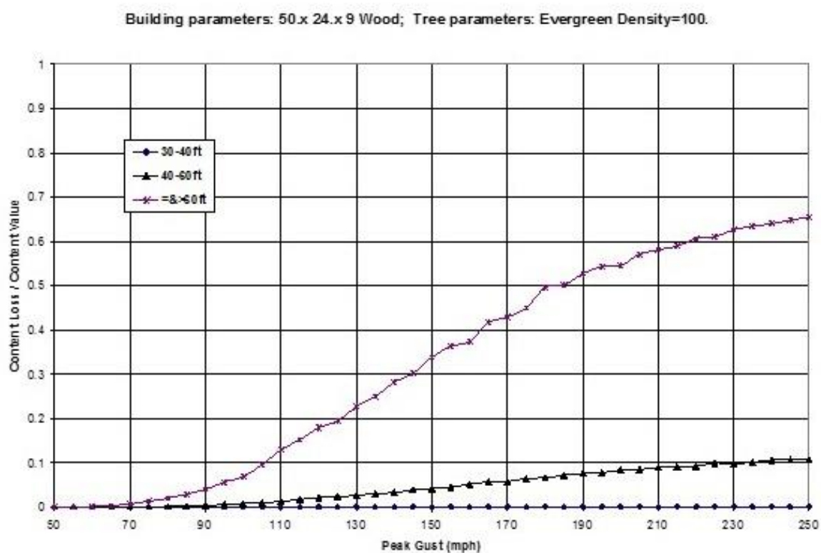
Figure 8-20 Dependence on Tree Height of Building (Upper) and Contents (Lower) Loss Functions
