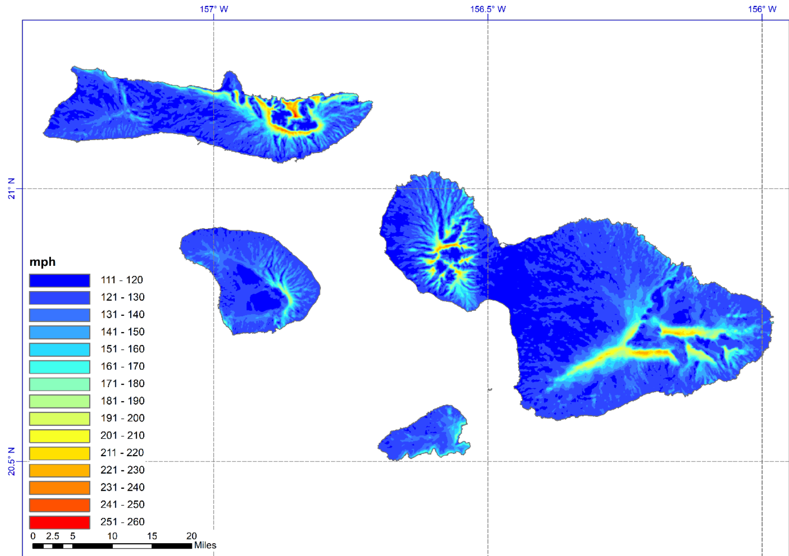
Figure 10-47 Peak gust wind speed map for a return period of 3,000-years for the islands of Maui, Molokai, Lanai, and Kaho'olawe. Modeled gust wind speeds include the effects of topography.
