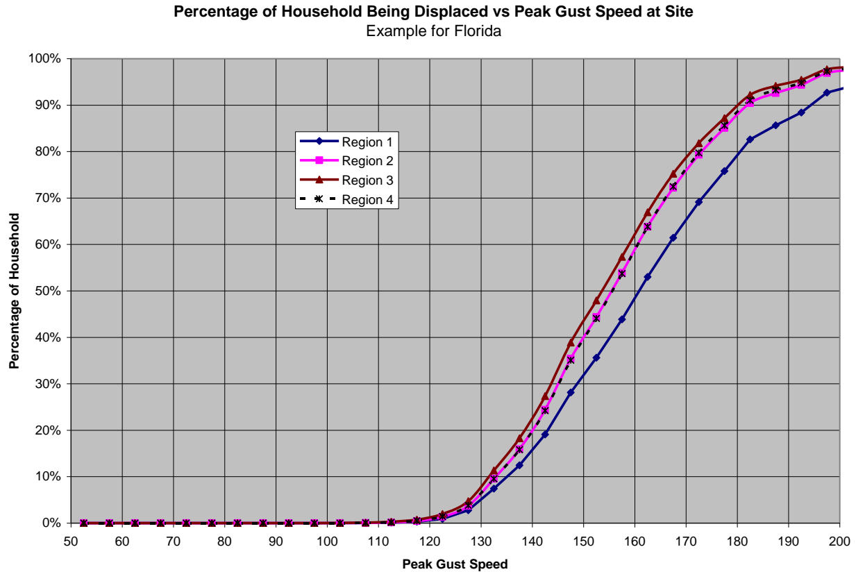
Figure 7-7 Example of Computed Percentage of Household Being Displaced as a Function of Peak Gust Wind Speed at Site
