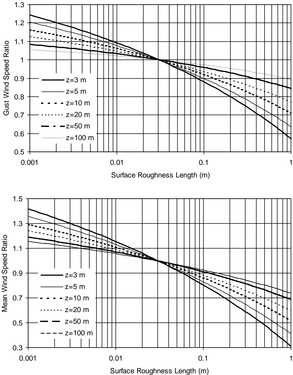
Figure 4-72 Wind Speed Ratios as a Function of Surface Roughness for Various Heights
