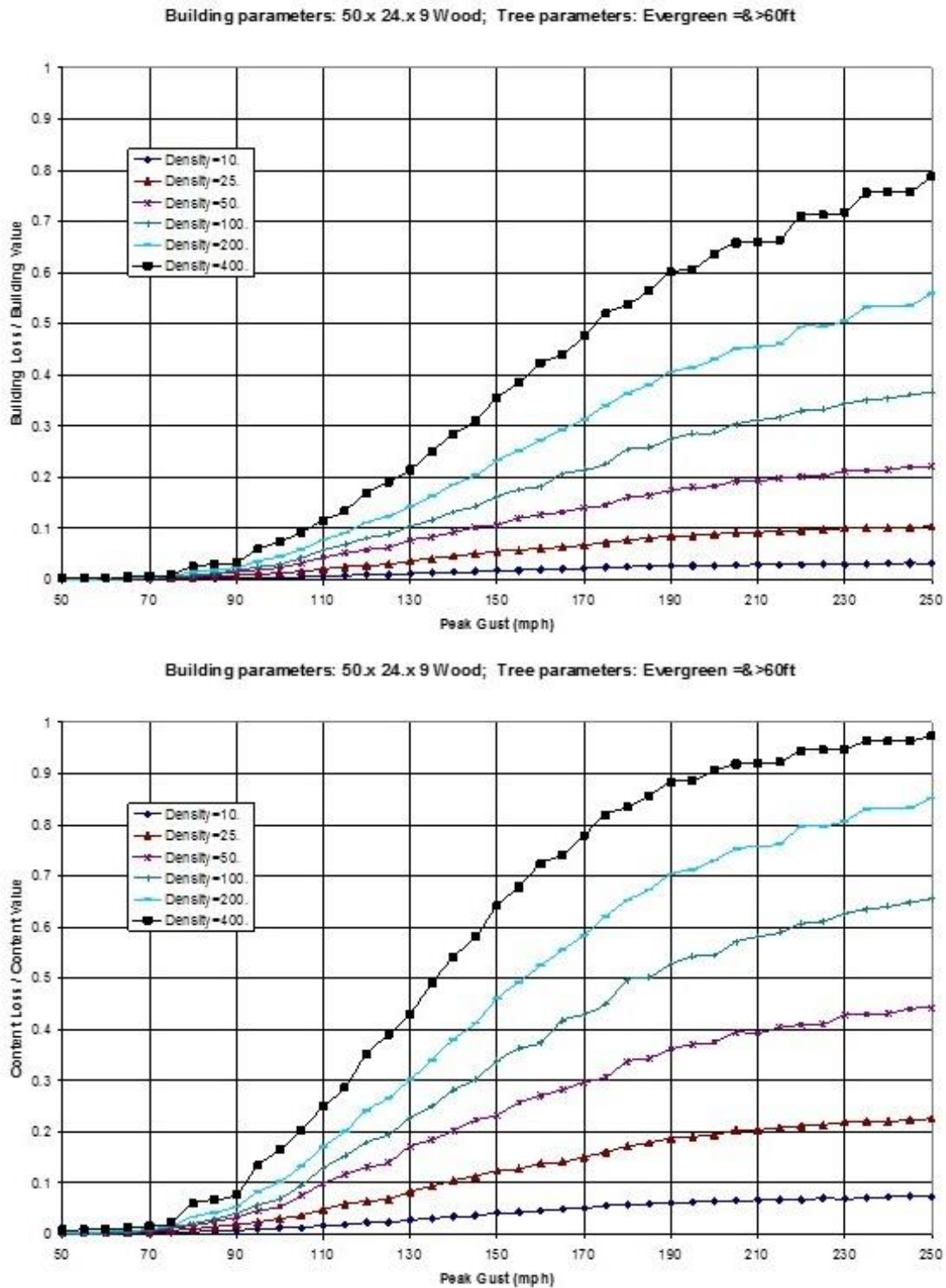
Figure 8-19 Dependence on Tree Density of Building (Upper) and Contents (Lower) Loss Functions
