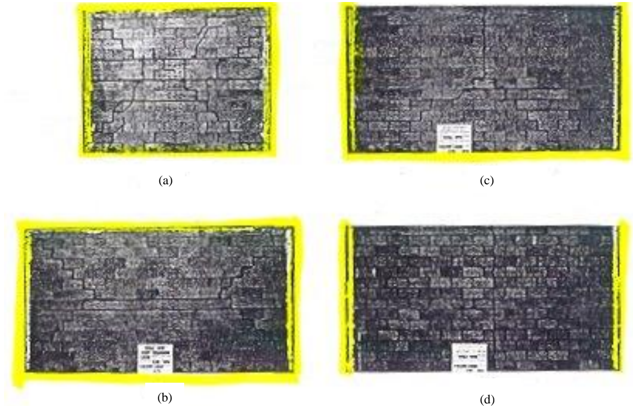
Figure 5-74 Typical Cracking Patterns for Various Wall Spans and Different Edge Support Conditions (Drysdale and Essawy, 1988)
