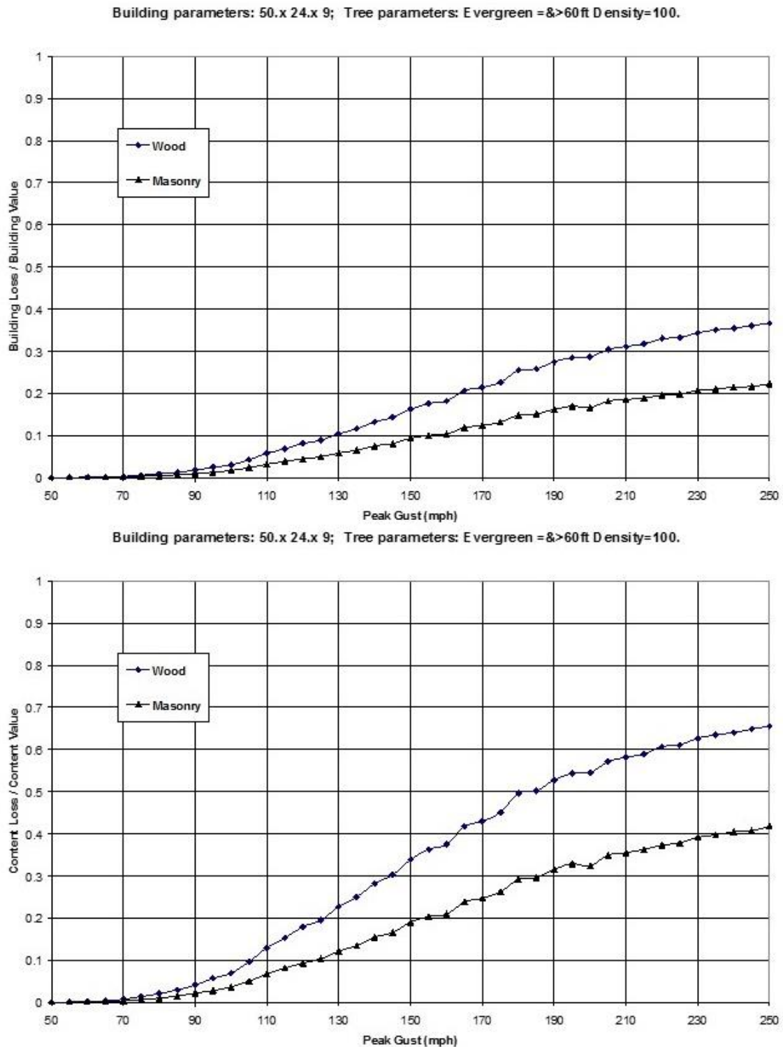
Figure 8-23 Dependence on Wall Type of Building (Upper) and Contents (Lower) Loss Functions
