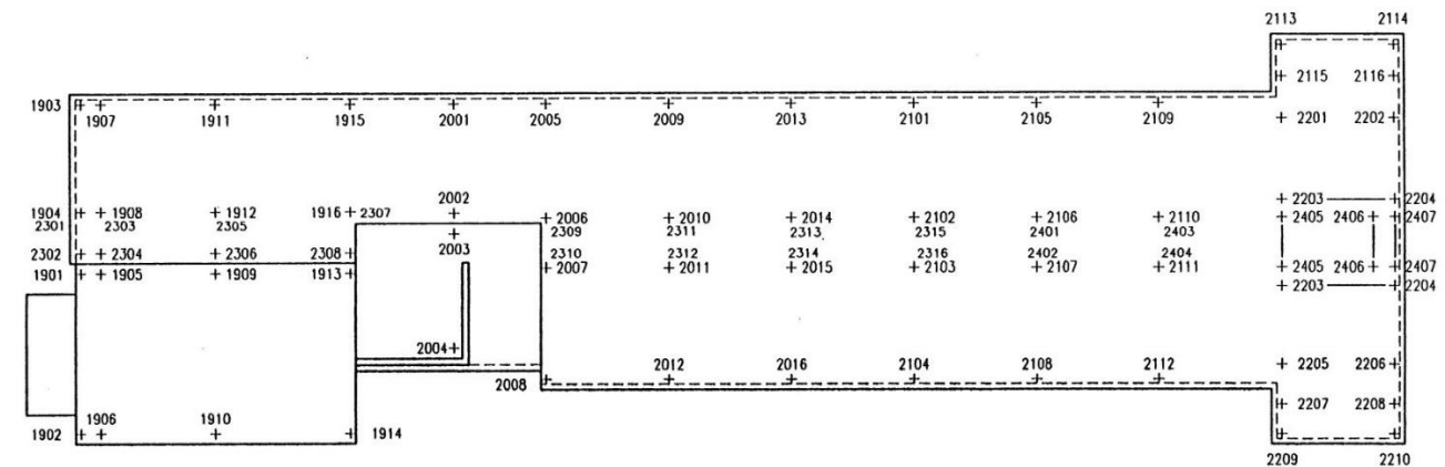
Figure 5-19 Plan View of School Showing Location of Truss Uplift Loads (North is towards top of page)
