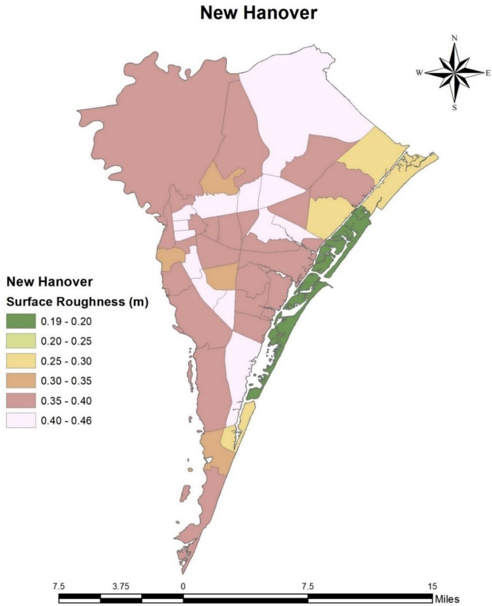
Figure 4-55 Census Tract-Averaged Roughness for New Hanover County, NC
