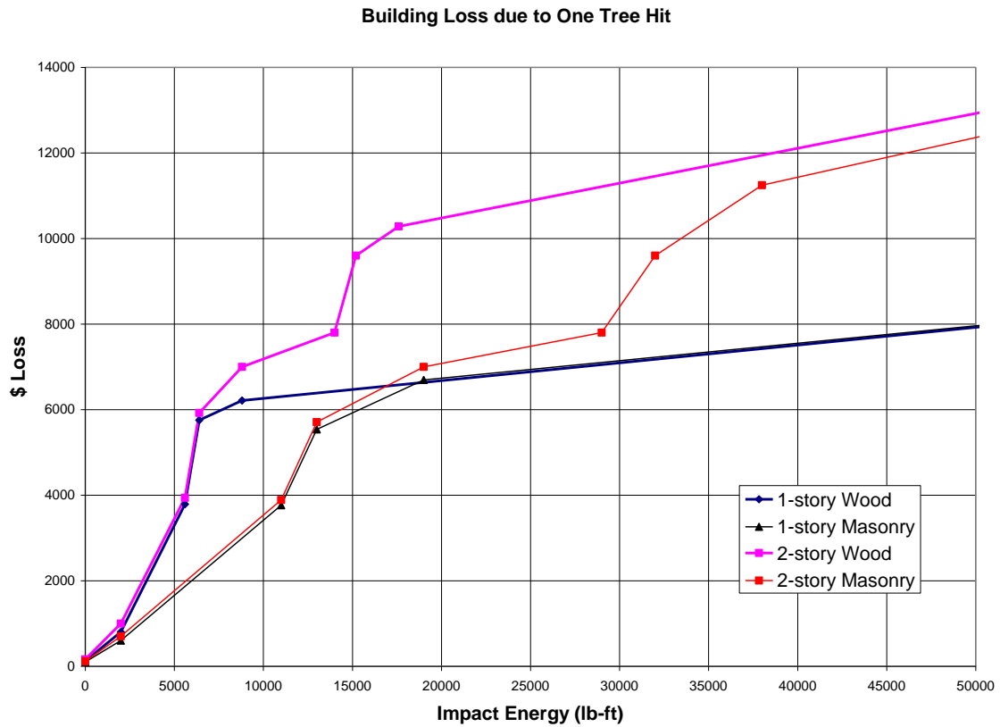
Figure 8-16 Building Repair Cost Estimates as Functions of Impact Energy
