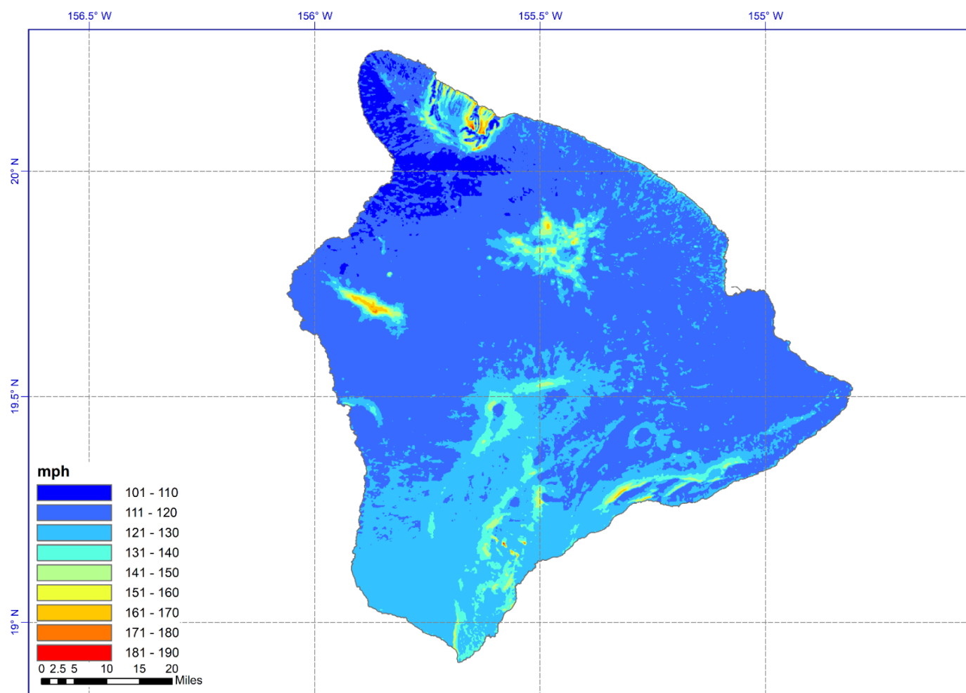
Figure 10-42 Peak gust wind speed map for a return period of 700-years for the island of Hawaii. Modeled gust wind speeds include the effects of topography.
