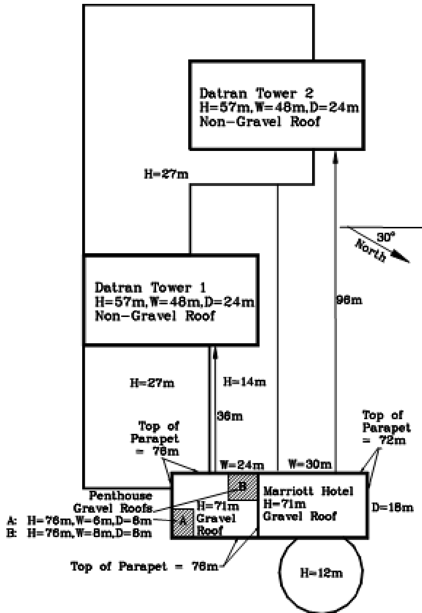
Figure 5-47 Approximate Plan of the Marriott-Datran Complex
