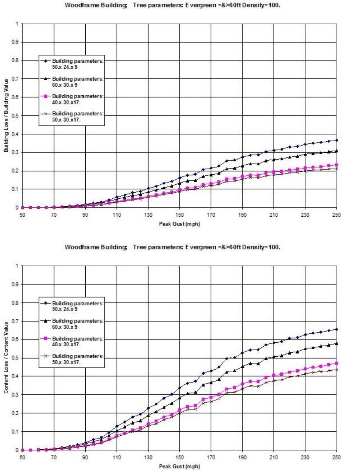
Figure 8-22 Dependence on Building Dimensions (ft) of Building (Upper) and Contents (Lower) Loss Functions
