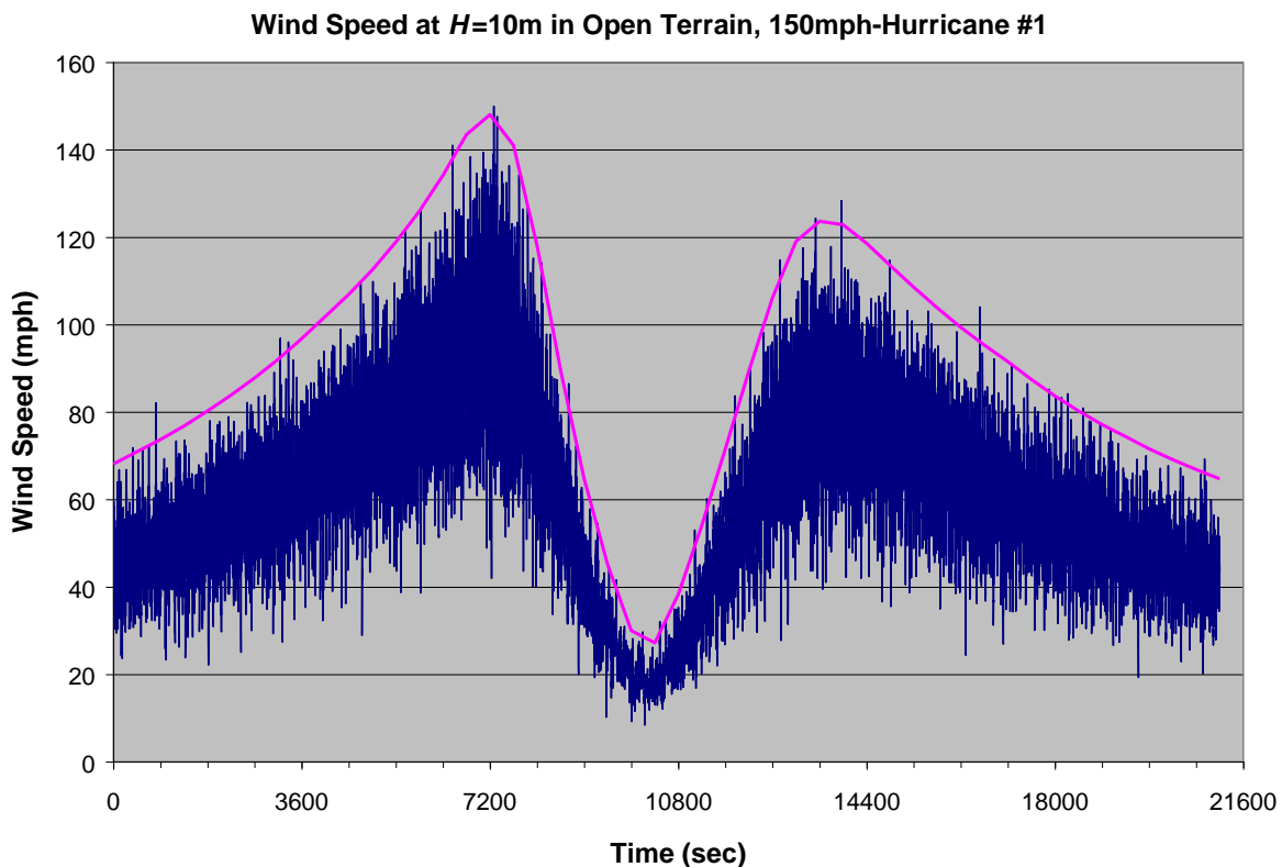
Figure 5-38 Example Hurricane Wind Speed Traces Used for the 150 mph Case – Hurricane #1
