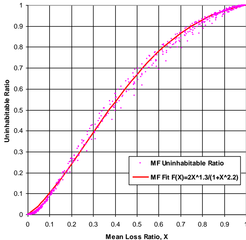
Figure 7-9 Uninhabitability as a Function of Mean Building Loss for Multi-Family Buildings
