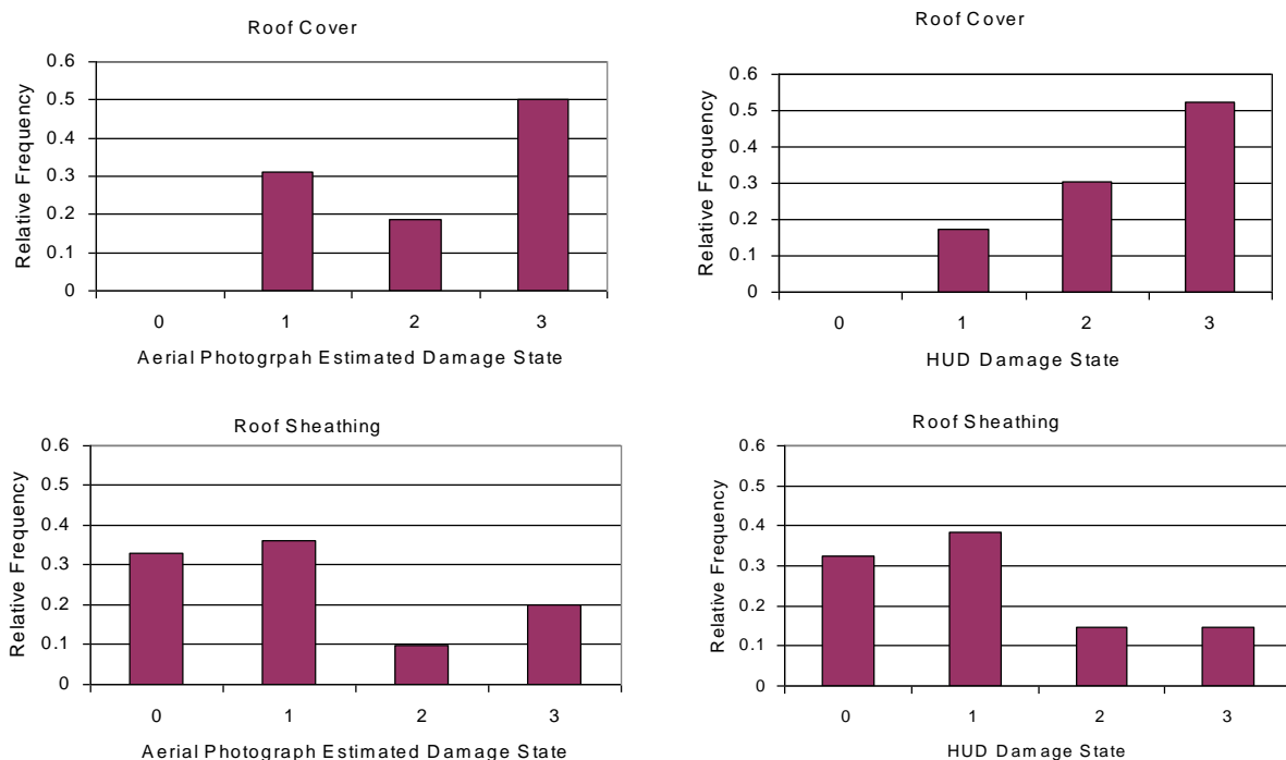
Figure 5-114 Comparison of Observed Damage States for Single-Story Gable Homes Obtained from Aerial Photography and HUD Damage Survey - Location of Photograph 3 (HUD Location D)
