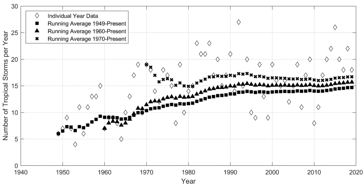
Figure 10-1 Number of tropical storms per year as reported in HURDAT2 in the Eastern and Central Pacific Ocean.
