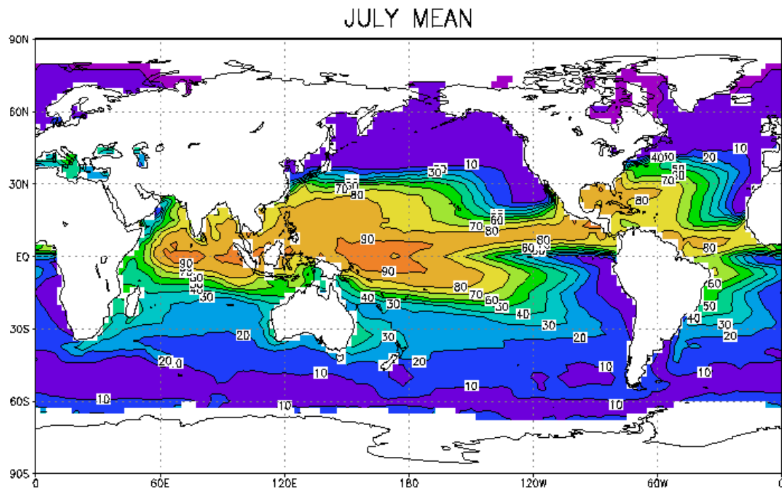
Figure 10-18 Mean exceedance probability maximum potential intensity at a point based on wind speed (maximum one-minute average surface wind speed, m/s) within 621 miles (1000 km) of the point in question for July.
