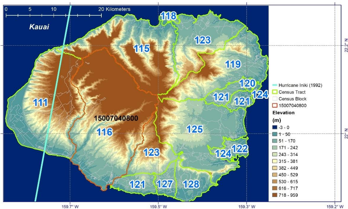
Figure 10-54 Modeled flat, open terrain peak gust winds for Hurricane Iniki (1992) at the census tract centroids of Kauai.
