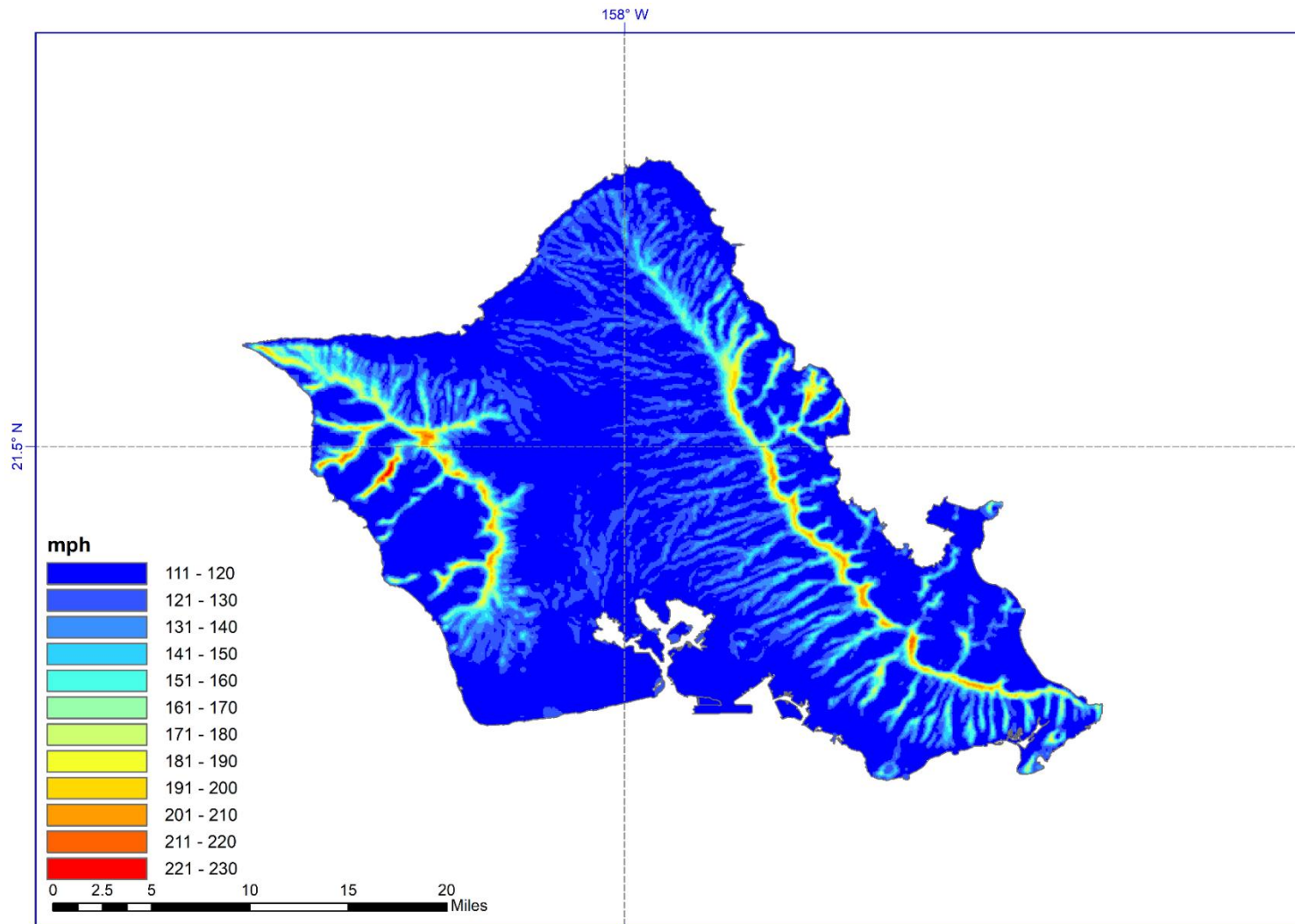
Figure 10-44 Peak gust wind speed map for a return period of 700-years for the island of Oahu. Modeled gust wind speeds include the effects of topography.
