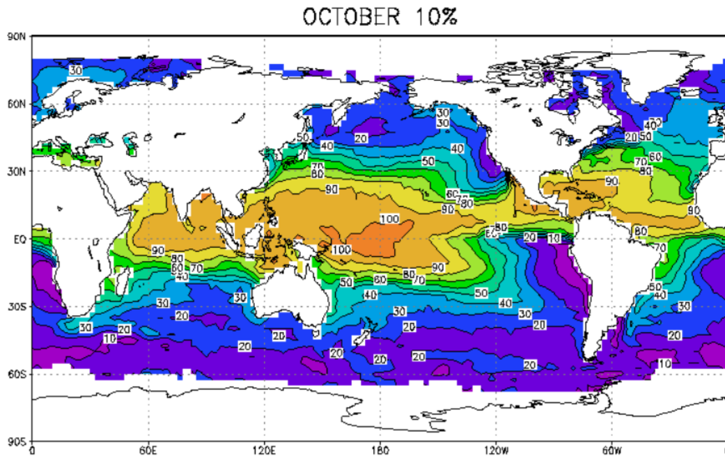
Figure 10-25 10% Exceedance probability maximum potential intensity at a point based on wind speed (maximum one-minute average surface wind speed, m/s) within 621 miles (1000 km) of the point in question for October.
