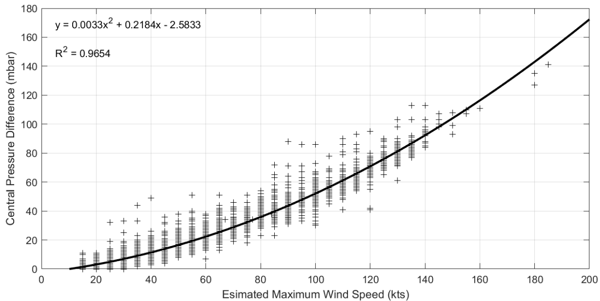
Figure 10-4 Central pressure difference vs maximum wind speed for events contained in the HURDAT2 database for the Eastern and Central Pacific Ocean.
