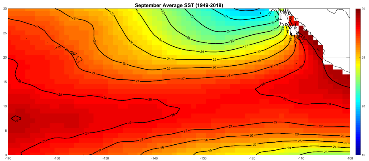
Figure 10-8 Mean September sea-surface temperature (°C)
