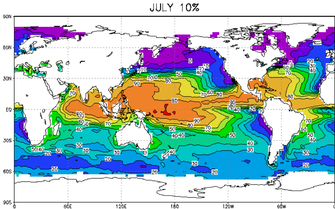
Figure 10-19 10% Exceedance probability maximum potential intensity at a point based on wind speed (maximum one-minute average surface wind speed, m/s) within 621 miles (1000 km) of the point in question for July.
