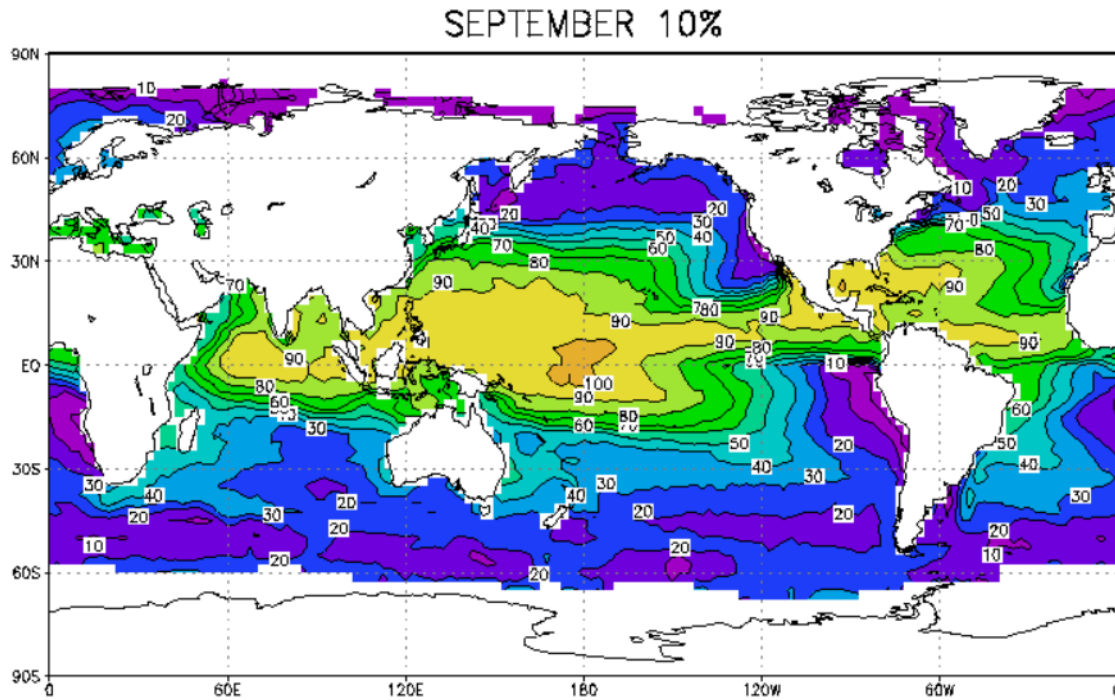
Figure 10-23 10% Exceedance probability maximum potential intensity at a point based on wind speed (maximum one-minute average surface wind speed, m/s) within 621 miles (1000 km) of the point in question for September.
