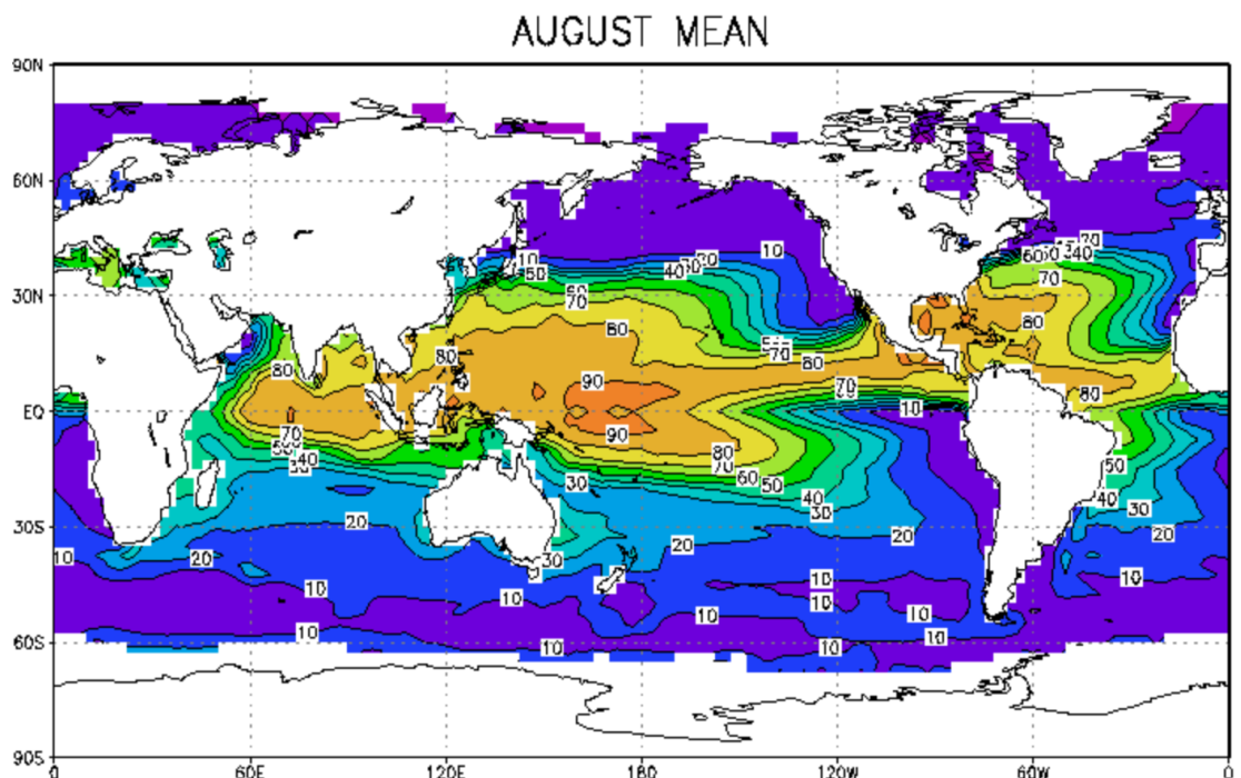
Figure 10-20 Mean exceedance probability maximum potential intensity at a point based on wind speed (maximum one-minute average surface wind speed, m/s) within 621 miles (1000 km) of the point in question for August
