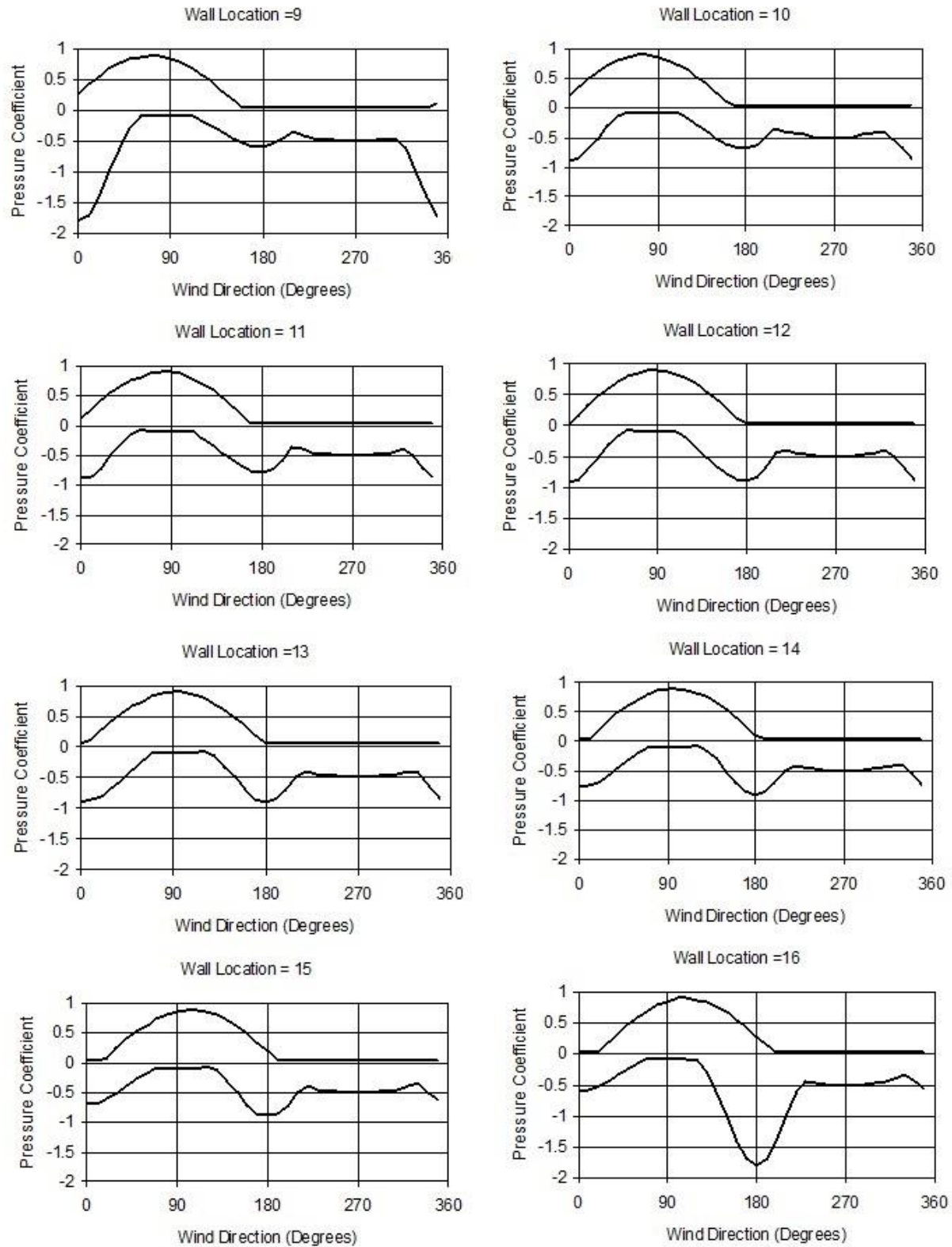
Figure 5-34 Maximum and Minimum Pressure Coefficients versus Wind Direction Used in Modeling of a Square High-Rise Building (continued)
