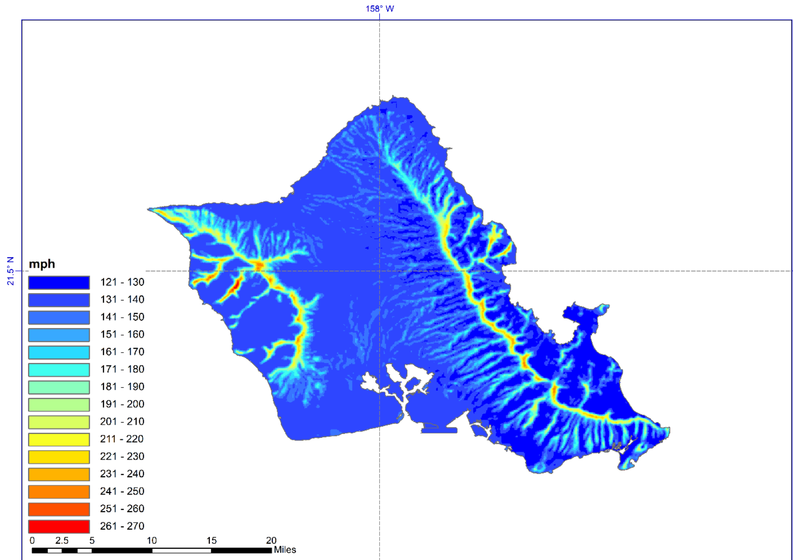
Figure 10-48 Peak gust wind speed map for a return period of 3,000-years for the island of Oahu. Modeled gust wind speeds include the effects of topography.
