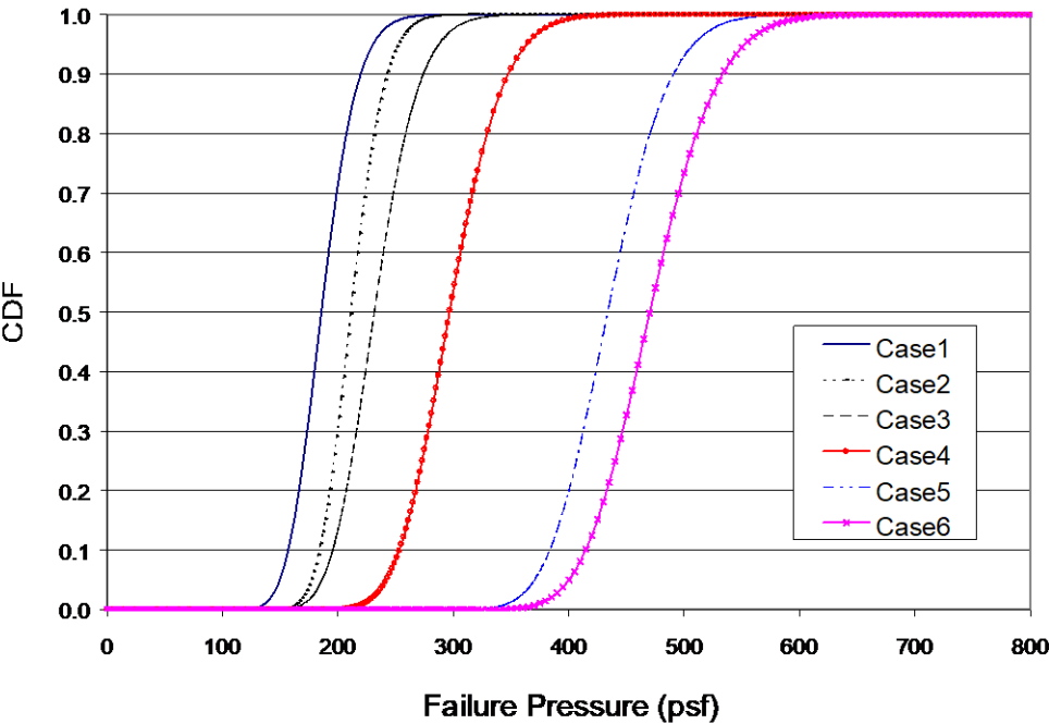
Figure 5-101 CDFs of Metal Deck Failure Pressures (Screw Connections)
