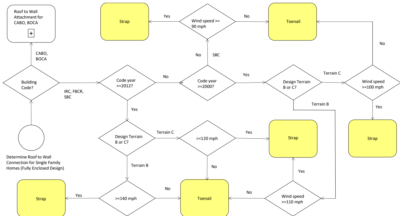
Figure 9-13 Roof-to-wall connection flowchart for one- and two-family dwellings with fully enclosed designs
