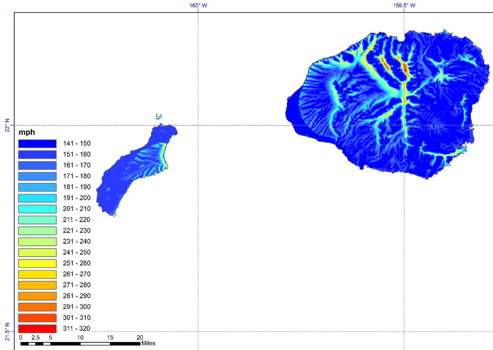
Figure 10-49 Peak gust wind speed map for a return period of 3,000-years for the islands of Kauai and Niihau. Modeled gust wind speeds include the effects of topography.
