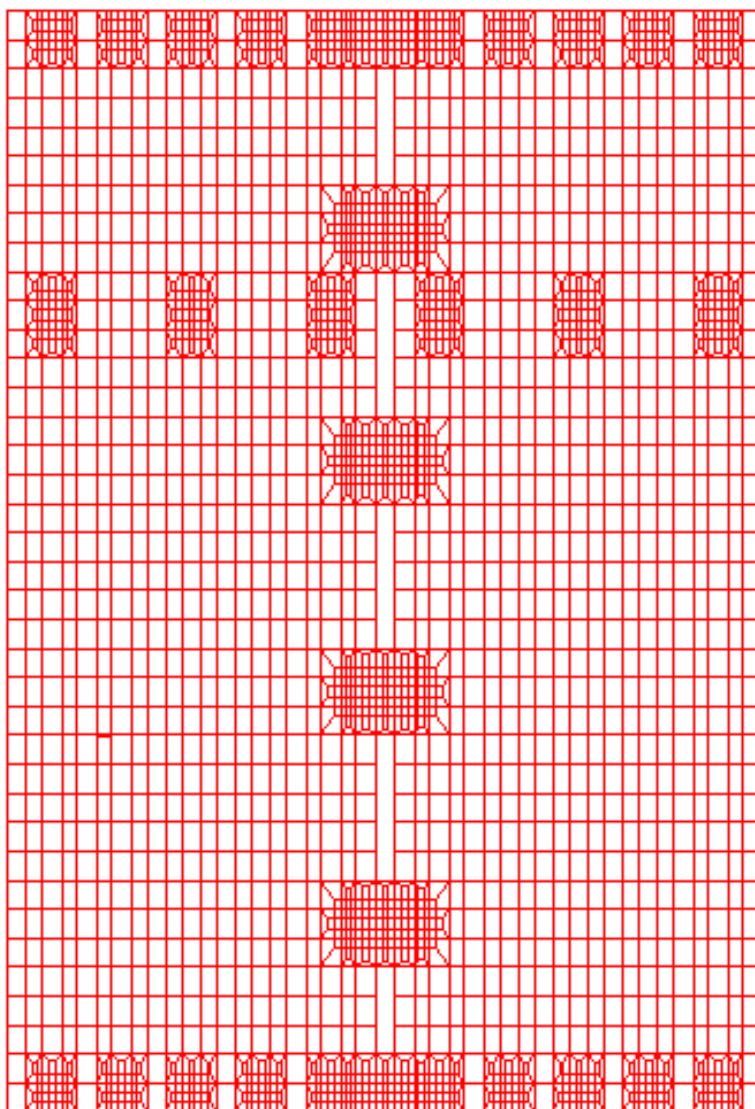
Figure 5-105 Finite Element Mesh of the Wall Panels
