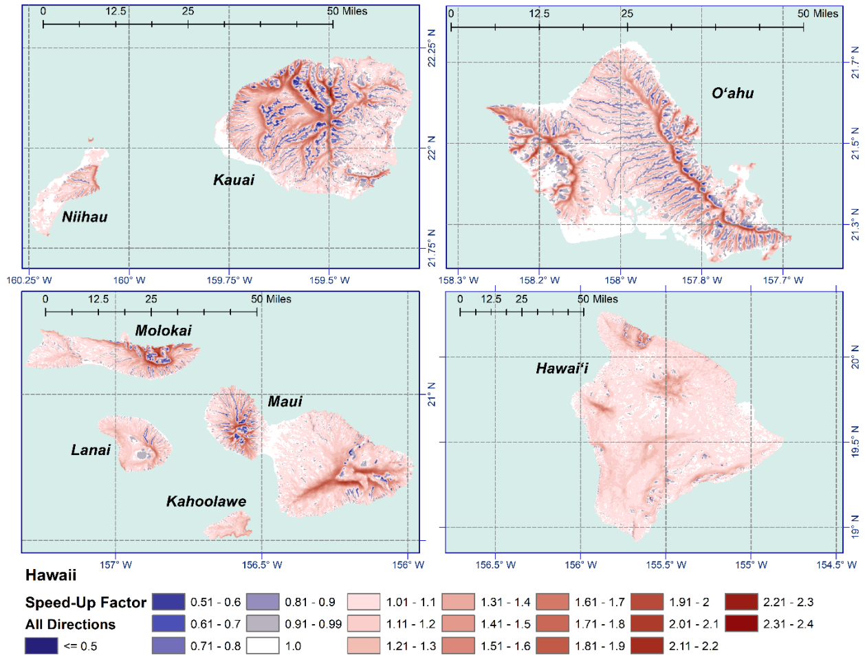
Figure 10-41 Speed-up factors (worst over all directions) for the Hawaiian Islands.
