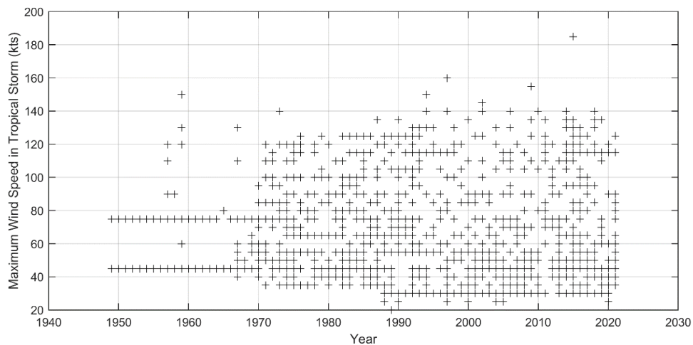
Figure 10-2 Maximum wind speed reported for each tropical storm in the HURDAT2 database for the Eastern and Central Pacific Ocean.
