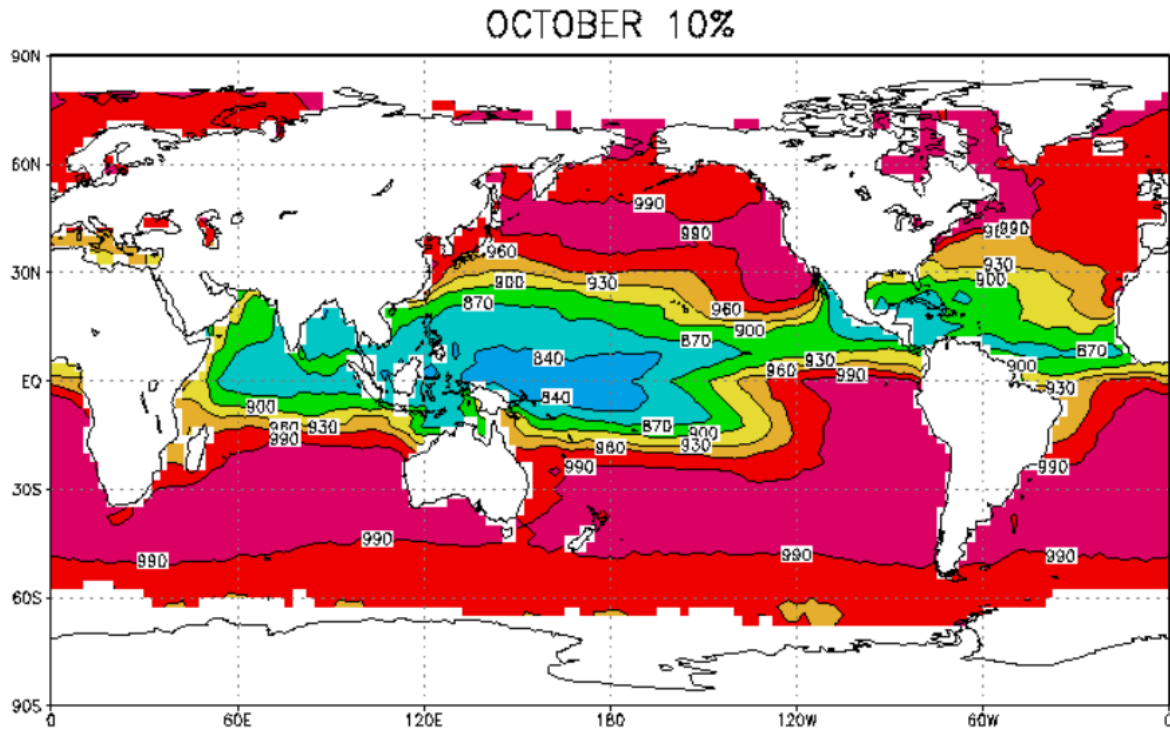
Figure 10-17 10% Exceedance probability maximum potential intensity at a point based on central pressure (hPa) within 621 miles (1000 km) of the point in question for October.
