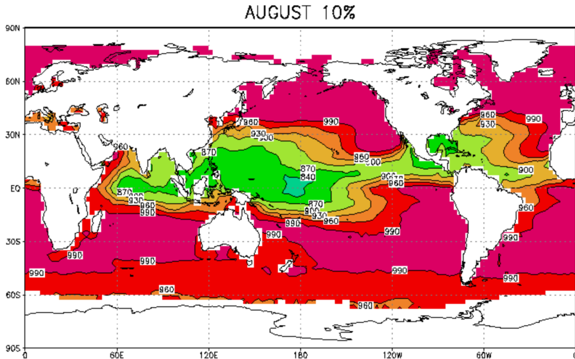
Figure 10-13 10% Exceedance probability maximum potential intensity at a point based on central pressure (hPa) within 621 miles (1000 km) of the point in question for August.
