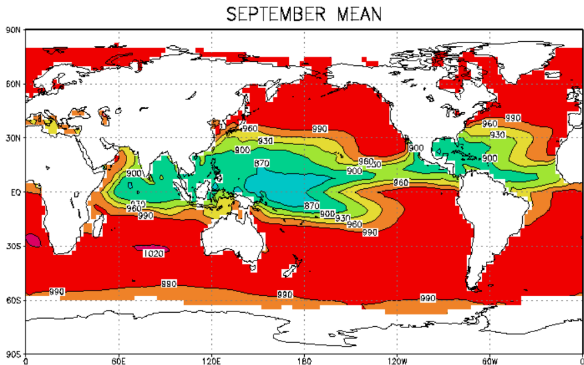
Figure 10-14 Mean exceedance probability maximum potential intensity at a point based on central pressure (hPa) within 621 miles (1000 km) of the point in question for September.
