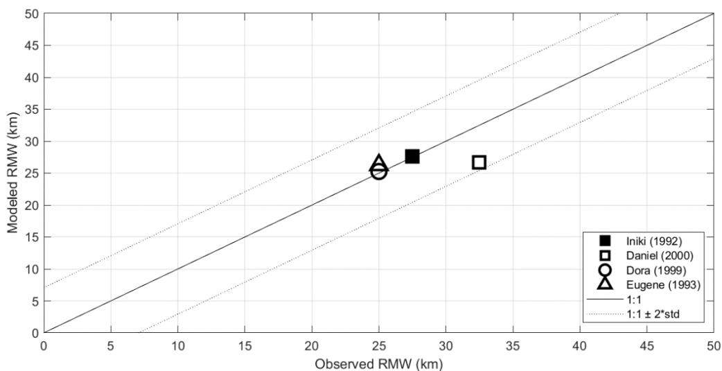
Figure 10-27 Modeled and observed radius of maximum winds for four tropical cyclones with information on RMW near the Hawaiian Islands.
