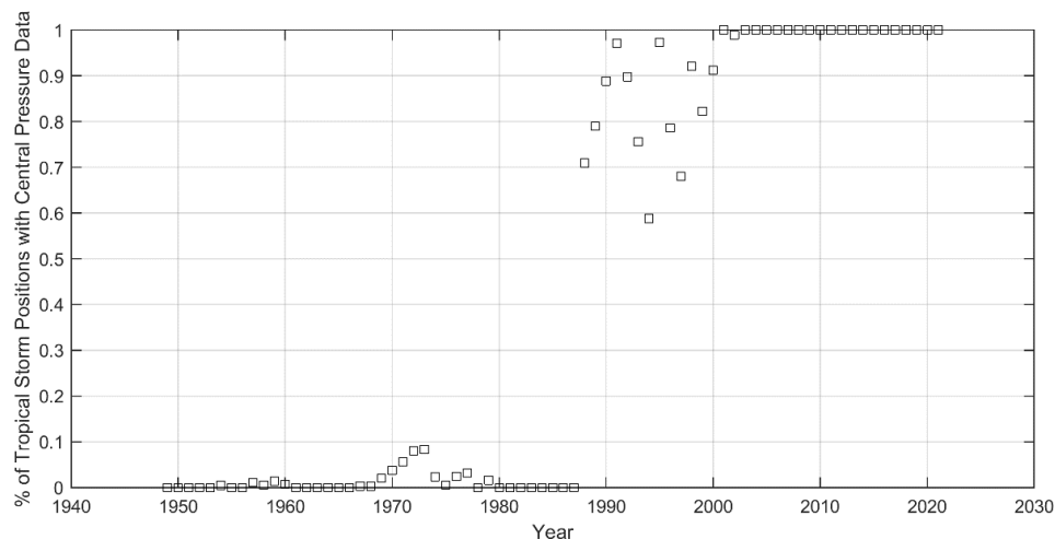
Figure 10-3 Percentage of storm track positions in the HURDAT2 database for the Eastern and Central Pacific Ocean with corresponding central pressure data.
