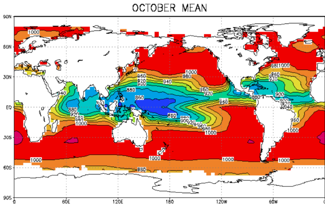
Figure 10-16 Mean exceedance probability maximum potential intensity at a point based on central pressure (hPa) within 621 miles (1000 km) of the point in question for October.
