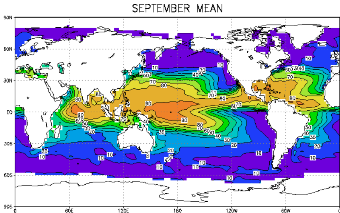
Figure 10-22 Mean exceedance probability maximum potential intensity at a point based on wind speed (one-minute average surface wind speed, m/s) within 621 miles (1000 km) of the point in question for September.
