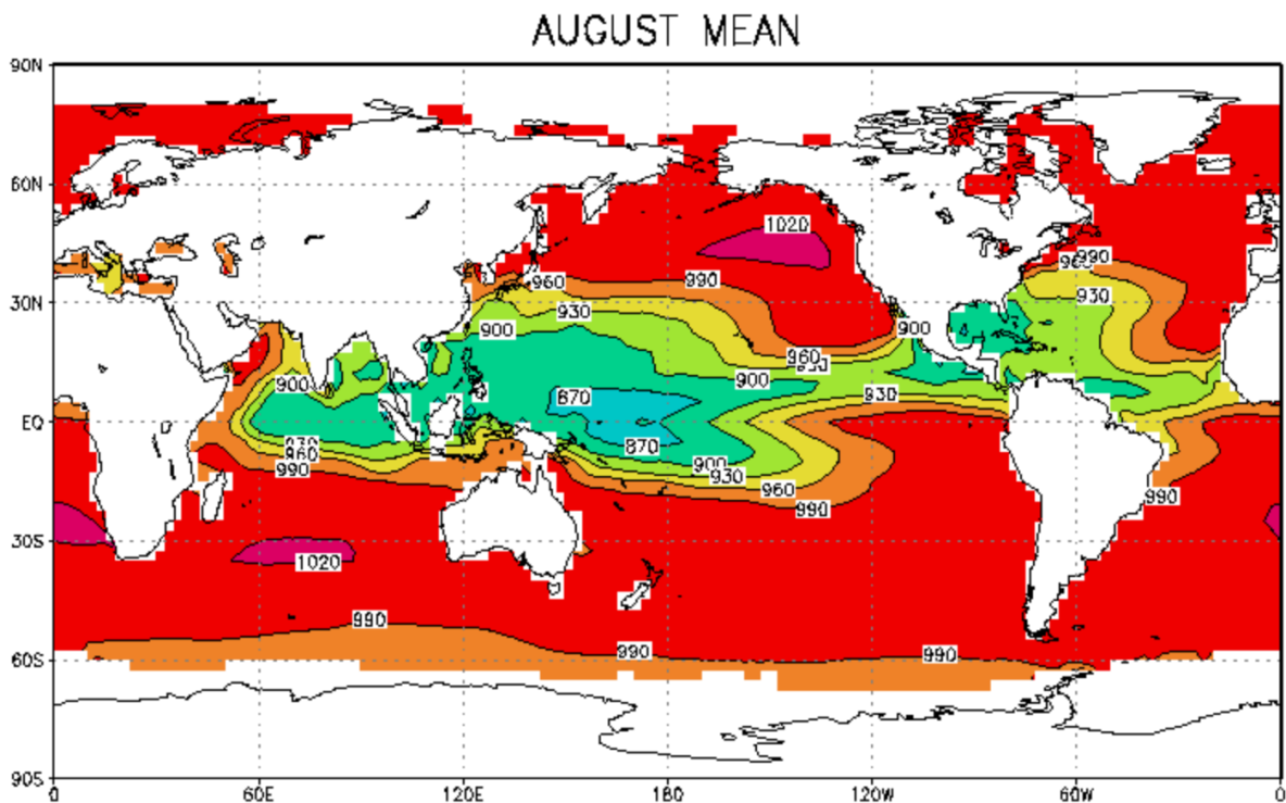
Figure 10-12 Mean exceedance probability maximum potential intensity at a point based on central pressure (hPa) within 621 miles (1000 km) of the point in question for August
