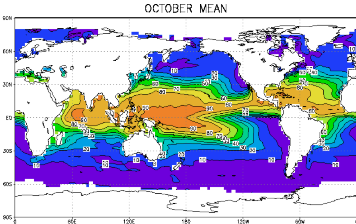
Figure 10-24 Mean exceedance probability maximum potential intensity at a point based on wind speed (maximum one-minute average surface wind speed, m/s) within 621 miles (1000 km) of the point in question for October.
