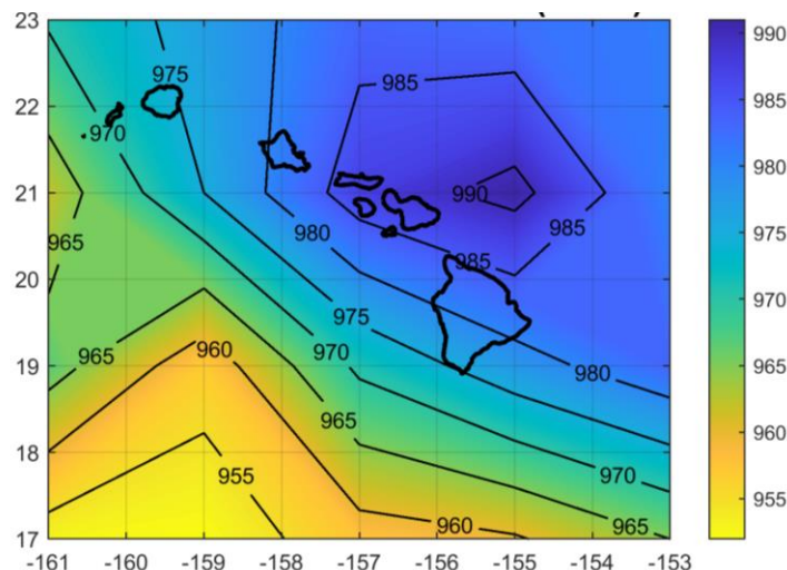
Figure 10-26 90% Percentile (10% Exceedance) Central Pressures around the Hawaiian Islands, based on all tropical cyclones passing within 250 km of a point during the period 1970 through 2021.
