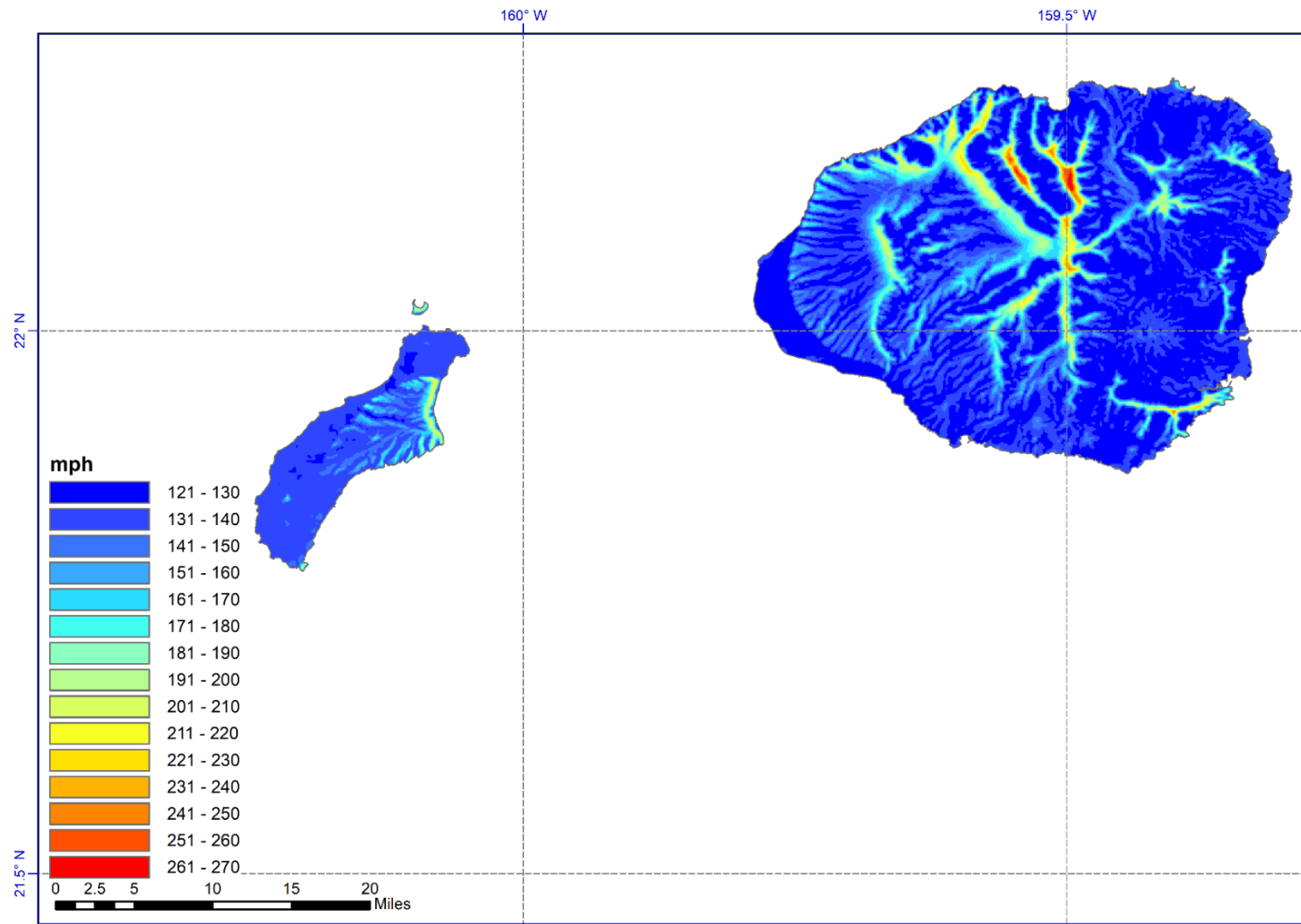
Figure 10-45 Peak gust wind speed map for a return period of 700-years for the islands of Kauai and Niihau. Modeled gust wind speeds include the effects of topography.
