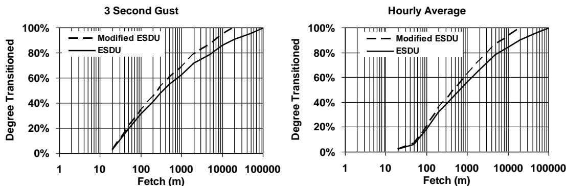
Figure 10-37 ESDU and modified ESDU wind speed transition functions at 10m elevation.
