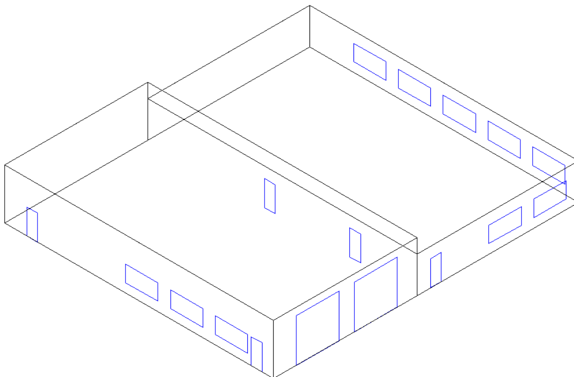
Figure 5-149 Fire Station Geometry Used in Study
