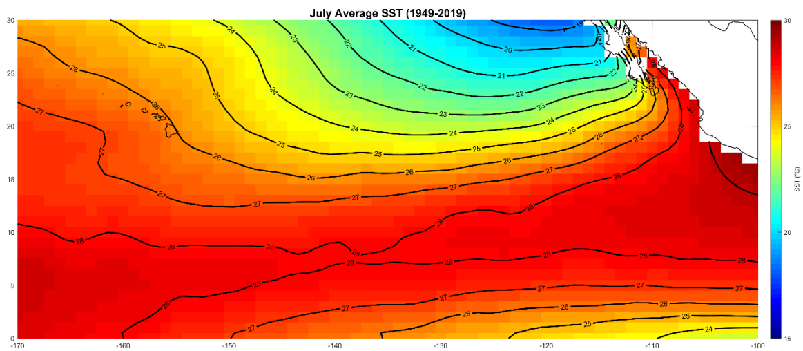
Figure 10-6 Mean July sea-surface temperature (°C).
