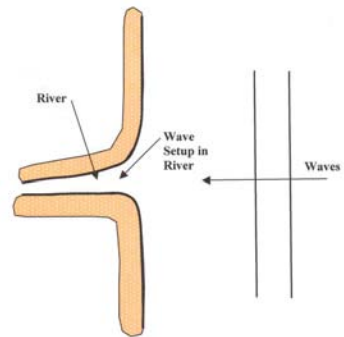
Setting 6. Wave Setup in River.
