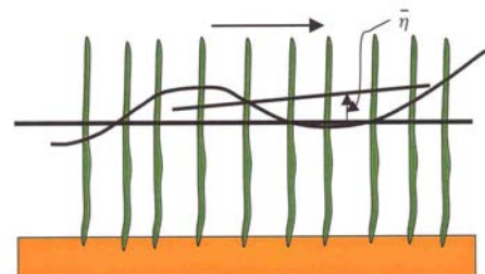
Setting 8. Wave Setup Through Vegetation.
