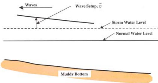
Setting 7. Wave Setup Over Muddy Bottom.
