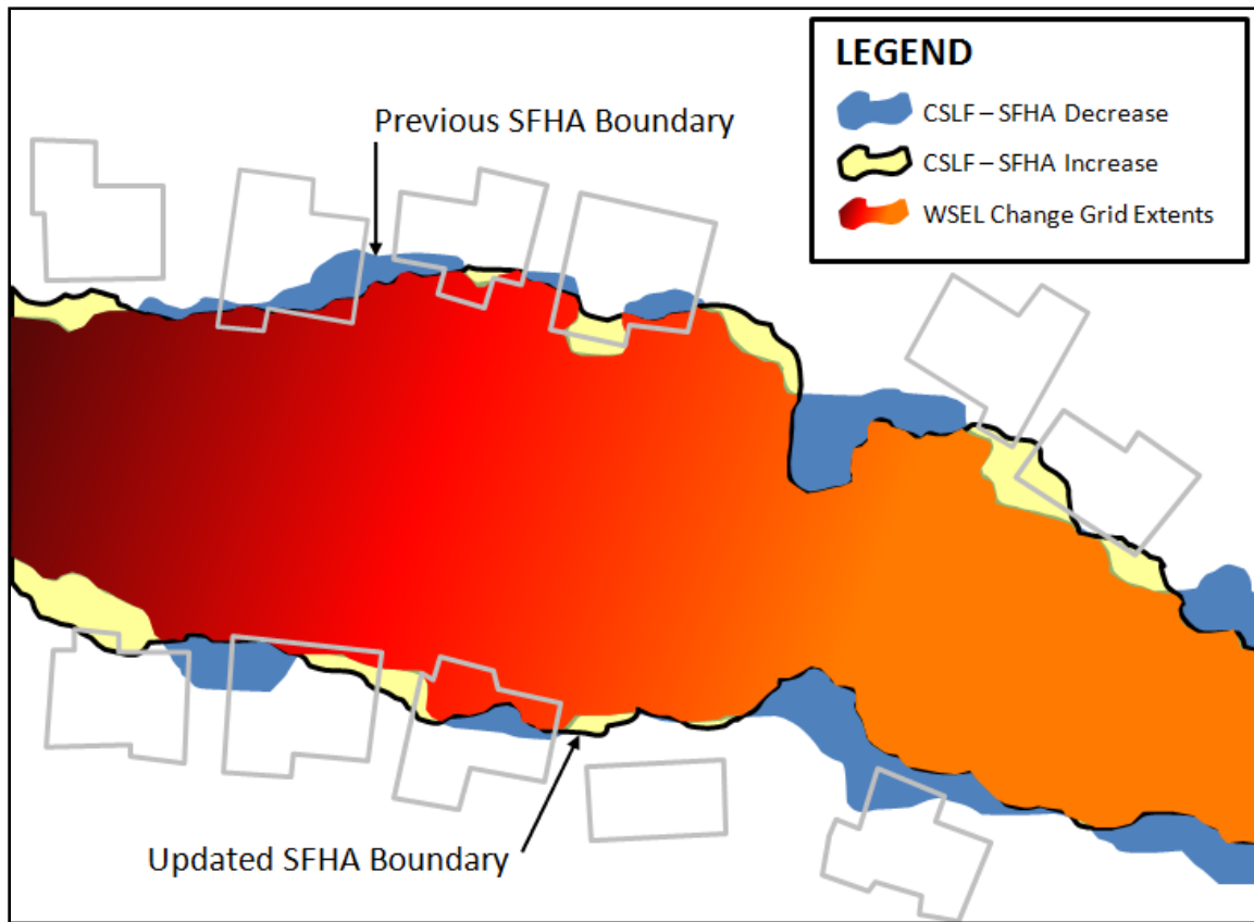
Figure 25: Water Surface Elevation Change Grid Extents
