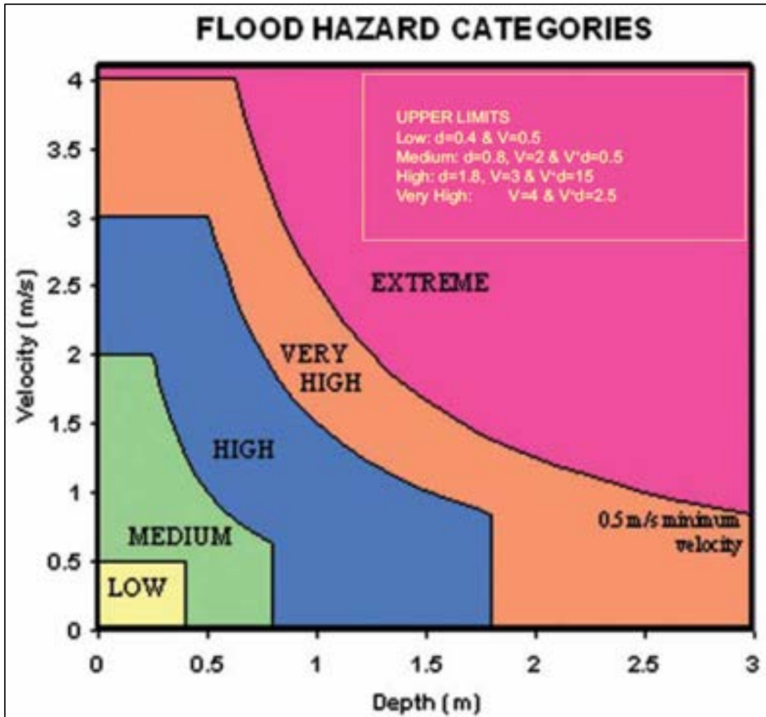
Figure 31: Example of Flood Severity Grid Classification
