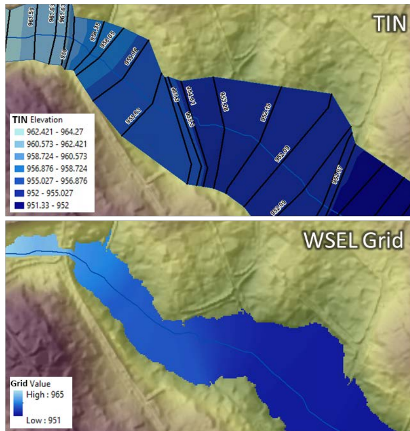
Figure 4: GRID Creation from a TIN
