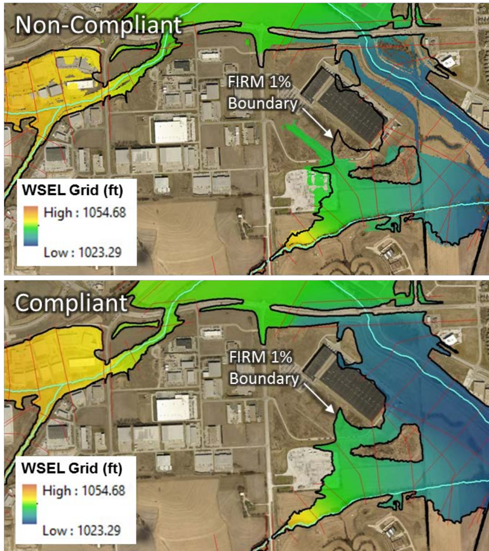
Figure 11: Comparison of Incorrect vs. Correct WSEL Grid Agreement to Mapping
