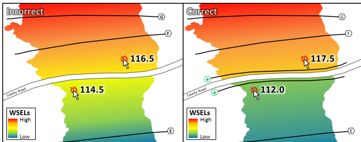
Figure 8: All Modeled Cross-Sections are Necessary for Accurate Grid Representation (WSEL Grid View)
