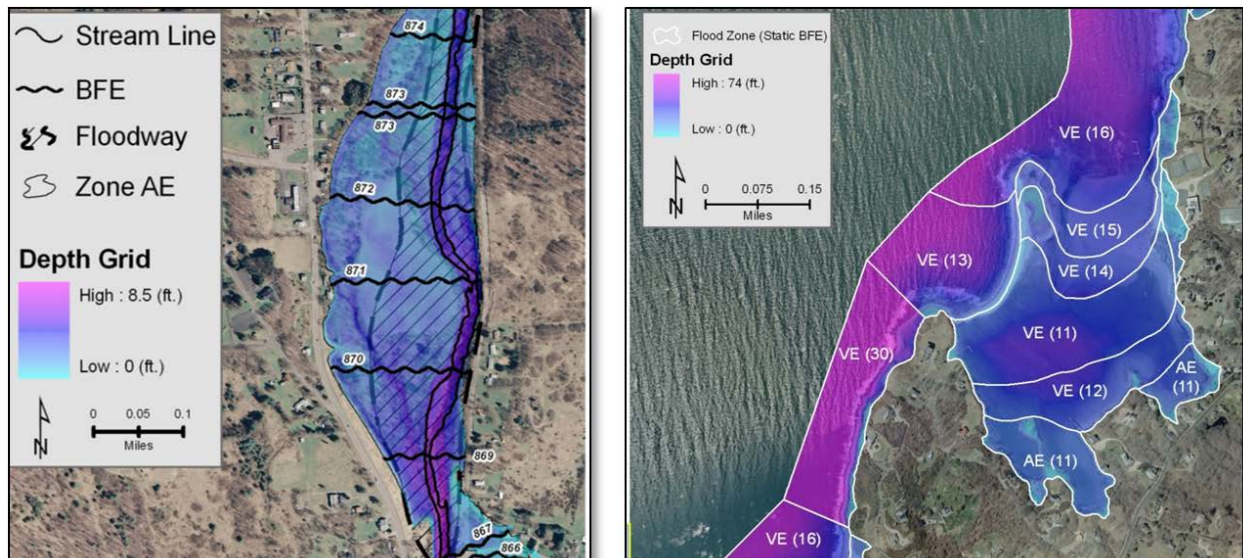
Figure 21: Examples of Riverine and Coastal Depth Grids
