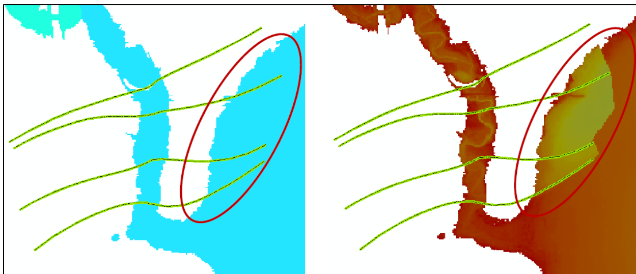
Figure 9: WSEL Grid Errors Resulting from Untrimmed Cross-Sections
