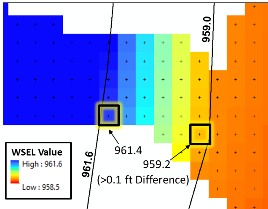
Figure 13: Example of Allowable WSEL Grid vs. Cross-Section Elevation Differences
