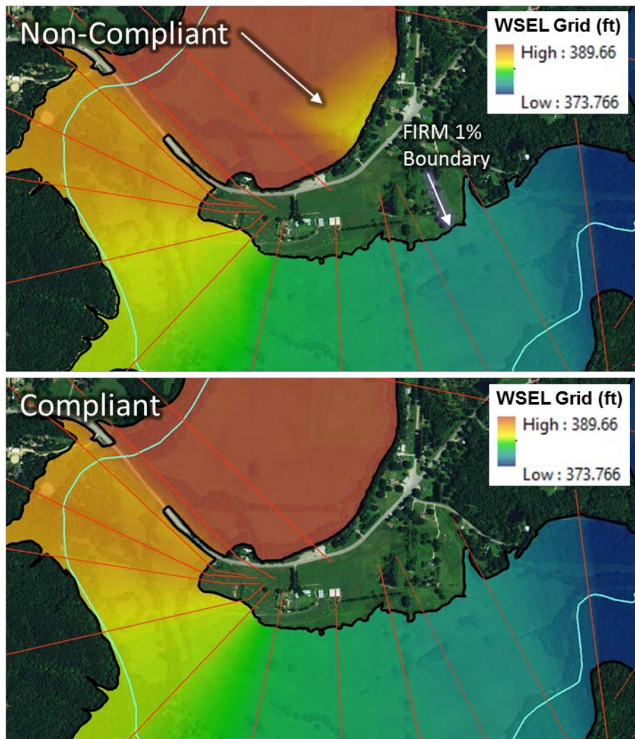
Figure 14: Importance of WSEL Grid Elevation Checks in Between Cross-Sections
