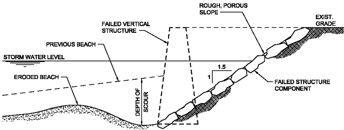
VERTICAL STRUCTURE FAILURE GEOMETRY
