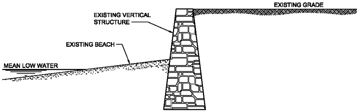
VERTICAL STRUCTURE GEOMETRY PRIOR TO FAILURE
