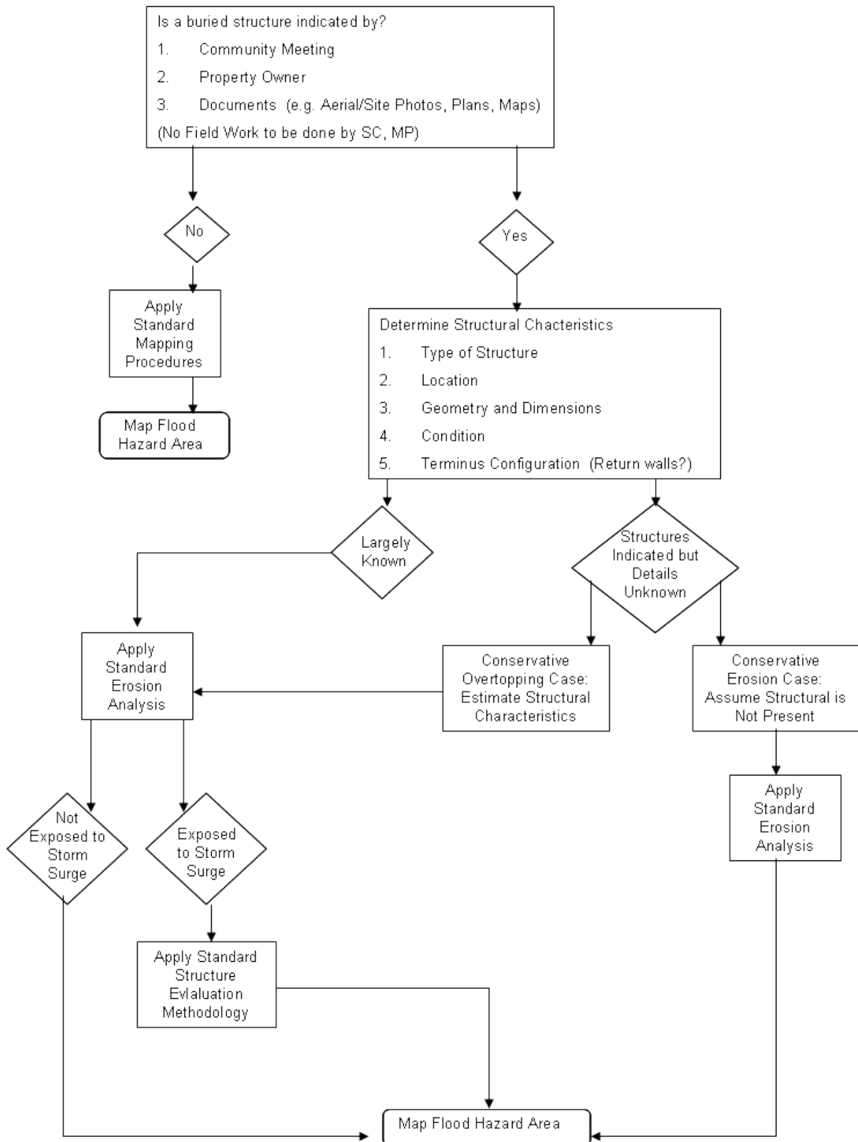
Figure 5: Methodology for Evaluating Buried Coastal Structures
