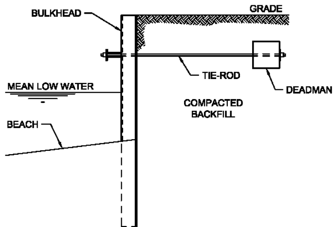
ANCHORED BULKHEAD
