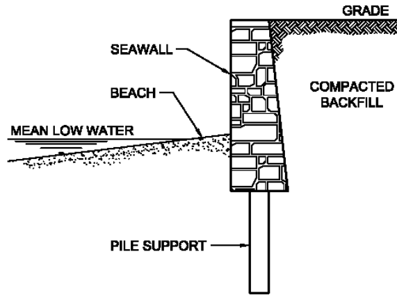
PILE SUPPORTED SEAWALL
