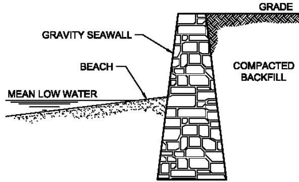
GRAVITY SEAWALL
