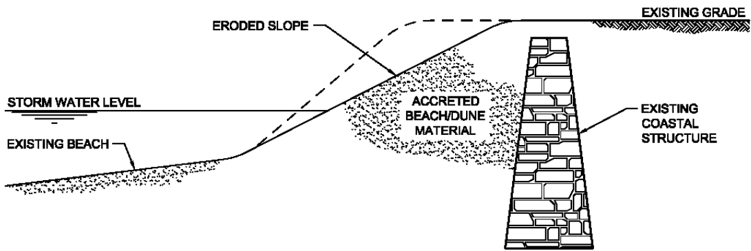
POST-EROSION GEOMETRY - BURIED STRUCTURE
