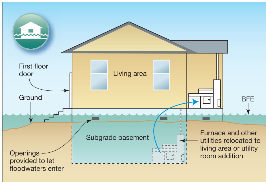
Figure 1-10. Wet floodproofed structure
